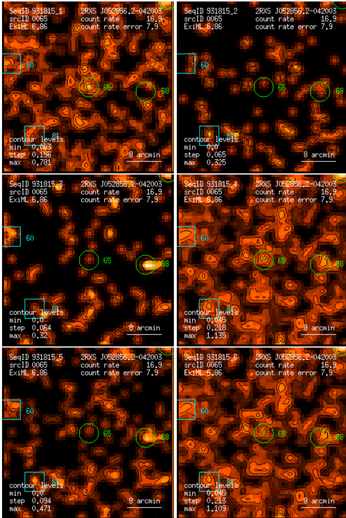
Figure 65: RASS 931815: detection 0065: band rate images, Gaussian filter: (1) PSPC channels 11 – 41, (2) 52 – 90, (3) 91 – 201, (4) 11 – 235, (5) 52 – 201, (6) 11 – 201. Broad band rates in counts/ks. Band rate contour levels in counts/ks/arcmin 2 .
