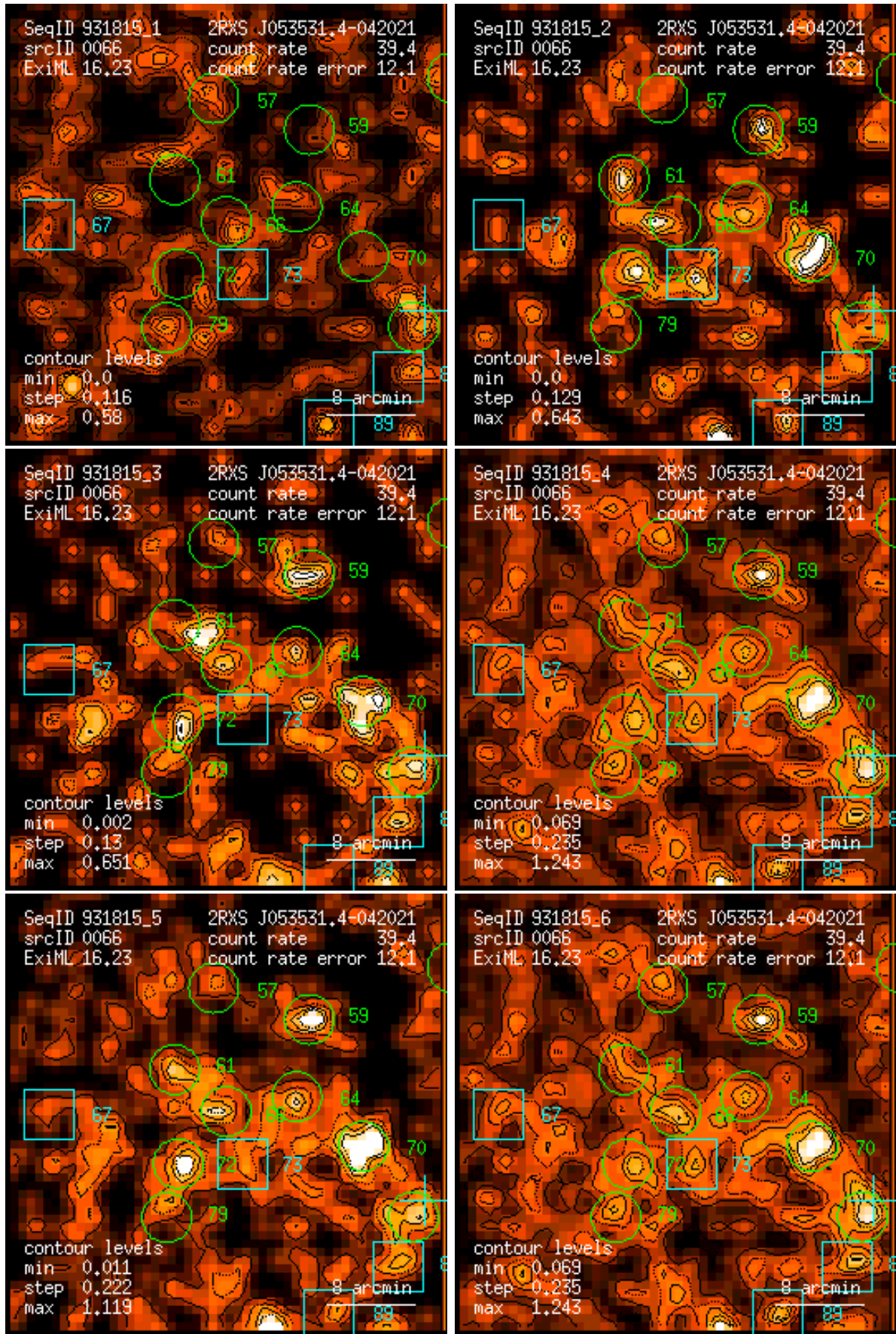
Figure 66: RASS 931815: detection 0066: band rate images, Gaussian filter: (1) PSPC channels 11 – 41, (2) 52 – 90, (3) 91 – 201, (4) 11 – 235, (5) 52 – 201, (6) 11 – 201. Broad band rates in counts/ks. Band rate contour levels in counts/ks/arcmin 2 .
