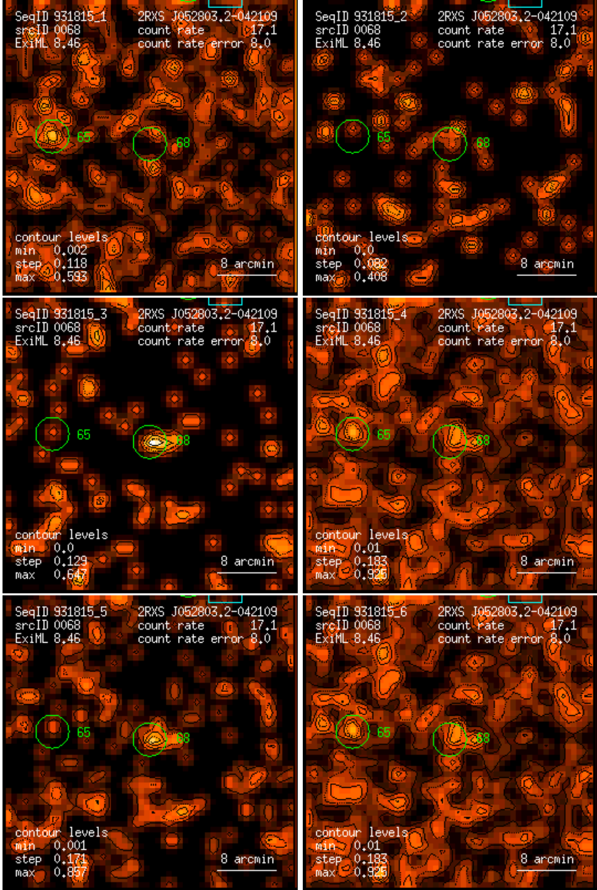
Figure 68: RASS 931815: detection 0068: band rate images, Gaussian filter: (1) PSPC channels 11 – 41, (2) 52 – 90, (3) 91 – 201, (4) 11 – 235, (5) 52 – 201, (6) 11 – 201. Broad band rates in counts/ks. Band rate contour levels in counts/ks/arcmin 2 .
