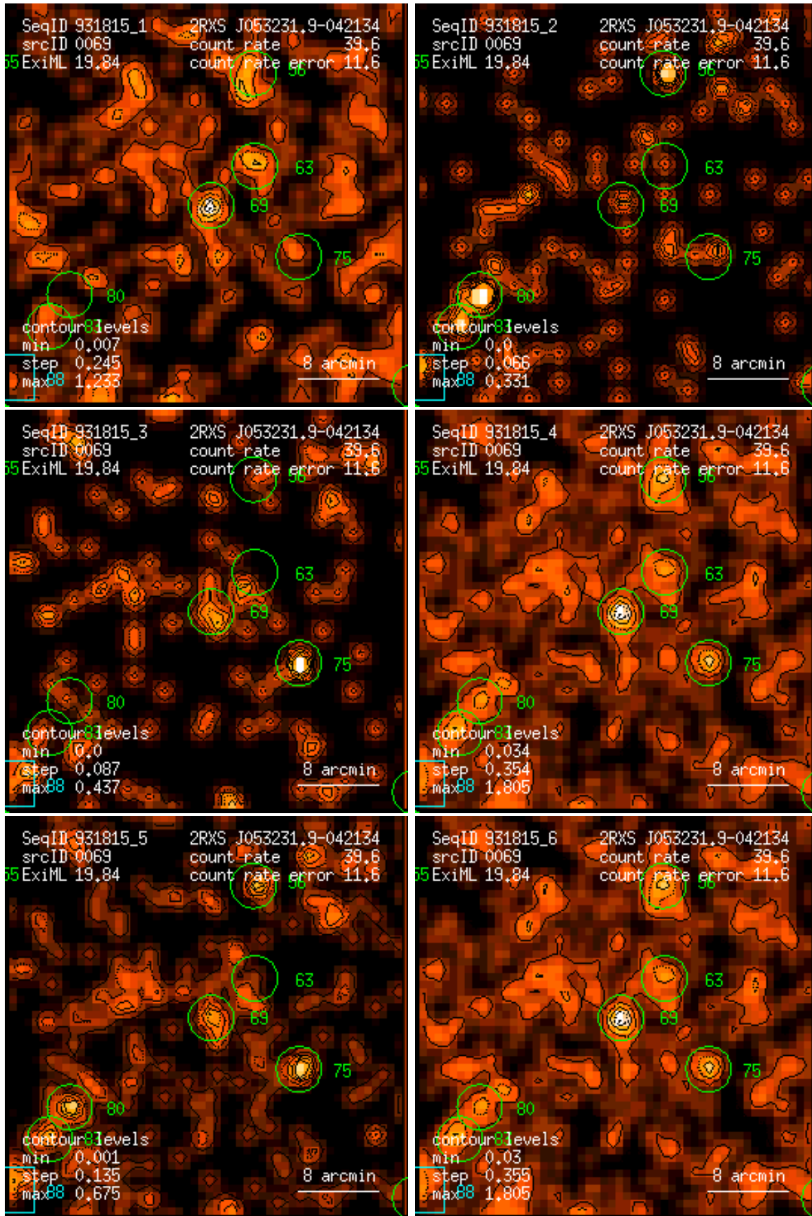
Figure 69: RASS 931815: detection 0069: band rate images, Gaussian filter: (1) PSPC channels 11 – 41, (2) 52 – 90, (3) 91 – 201, (4) 11 – 235, (5) 52 – 201, (6) 11 – 201. Broad band rates in counts/ks. Band rate contour levels in counts/ks/arcmin 2 .
