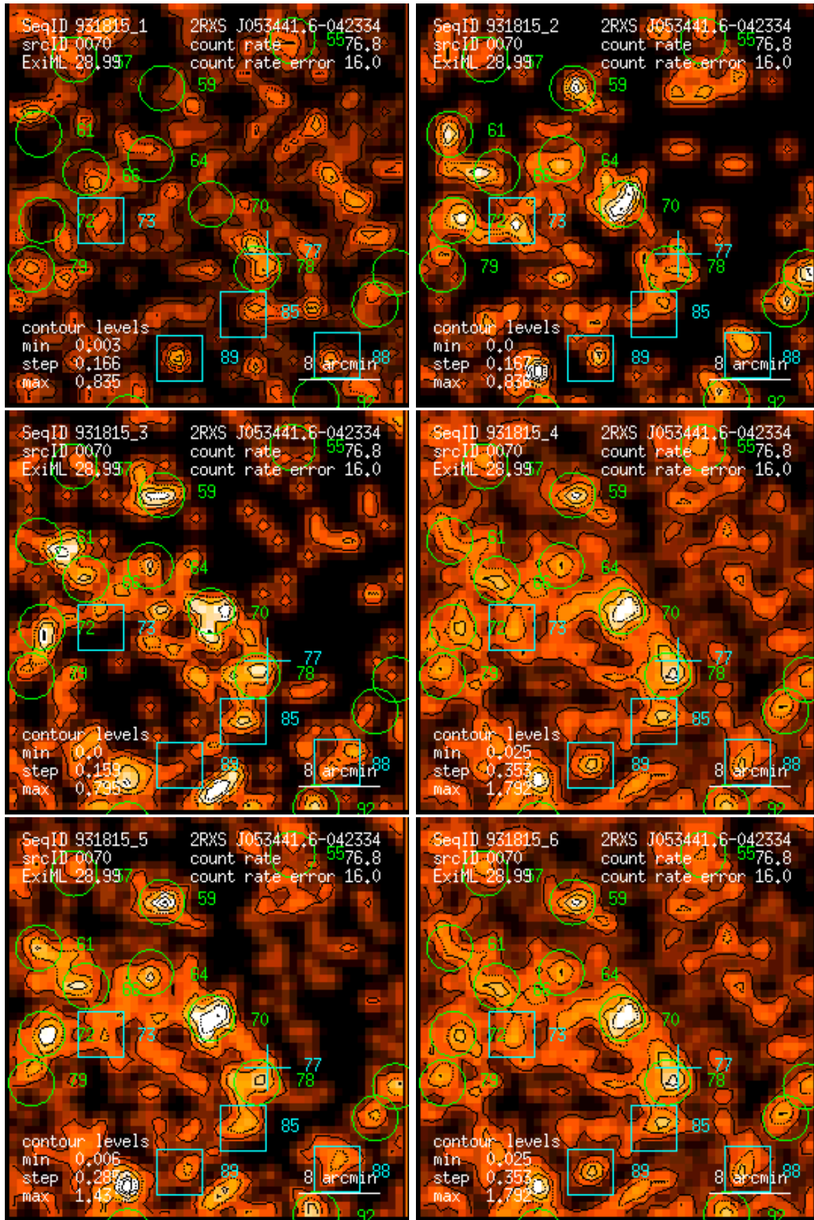
Figure 70: RASS 931815: detection 0070: band rate images, Gaussian filter: (1) PSPC channels 11 – 41, (2) 52 – 90, (3) 91 – 201, (4) 11 – 235, (5) 52 – 201, (6) 11 – 201. Broad band rates in counts/ks. Band rate contour levels in counts/ks/arcmin 2 .
