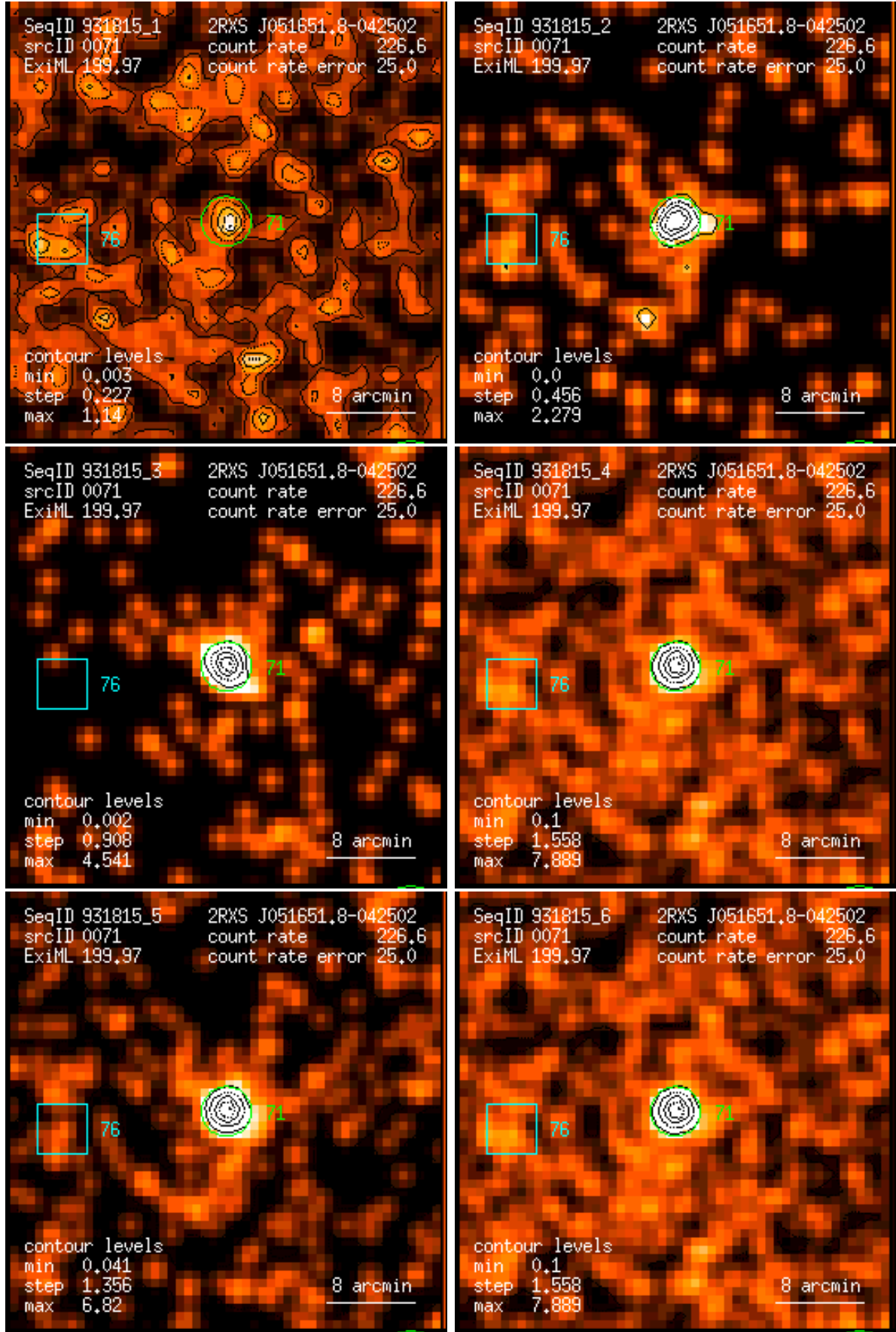
Figure 71: RASS 931815: detection 0071: band rate images, Gaussian filter: (1) PSPC channels 11 – 41, (2) 52 – 90, (3) 91 – 201, (4) 11 – 235, (5) 52 – 201, (6) 11 – 201. Broad band rates in counts/ks. Band rate contour levels in counts/ks/arcmin 2 .
