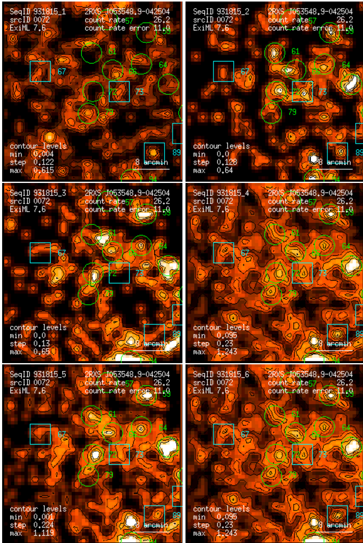
Figure 72: RASS 931815: detection 0072: band rate images, Gaussian filter: (1) PSPC channels 11 – 41, (2) 52 – 90, (3) 91 – 201, (4) 11 – 235, (5) 52 – 201, (6) 11 – 201. Broad band rates in counts/ks. Band rate contour levels in counts/ks/arcmin 2 .
