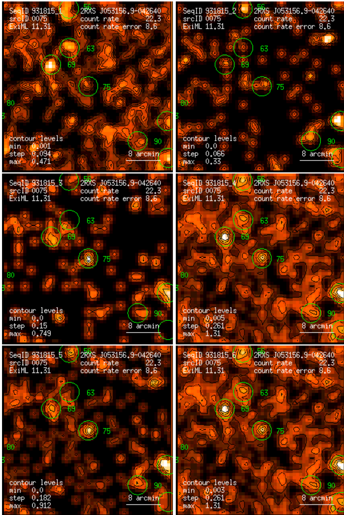
Figure 75: RASS 931815: detection 0075: band rate images, Gaussian filter: (1) PSPC channels 11 – 41, (2) 52 – 90, (3) 91 – 201, (4) 11 – 235, (5) 52 – 201, (6) 11 – 201. Broad band rates in counts/ks. Band rate contour levels in counts/ks/arcmin 2 .
