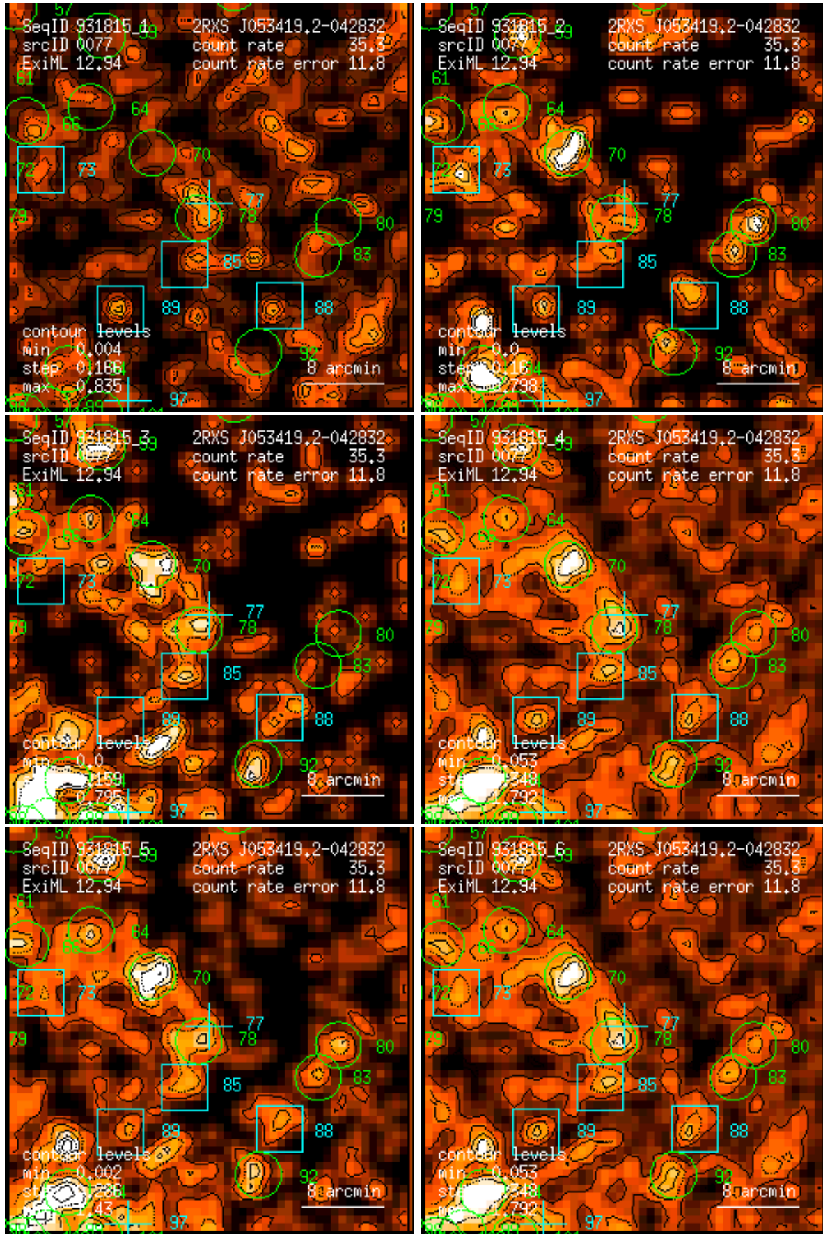
Figure 77: RASS 931815: detection 0077: band rate images, Gaussian filter: (1) PSPC channels 11 – 41, (2) 52 – 90, (3) 91 – 201, (4) 11 – 235, (5) 52 – 201, (6) 11 – 201. Broad band rates in counts/ks. Band rate contour levels in counts/ks/arcmin 2 .
