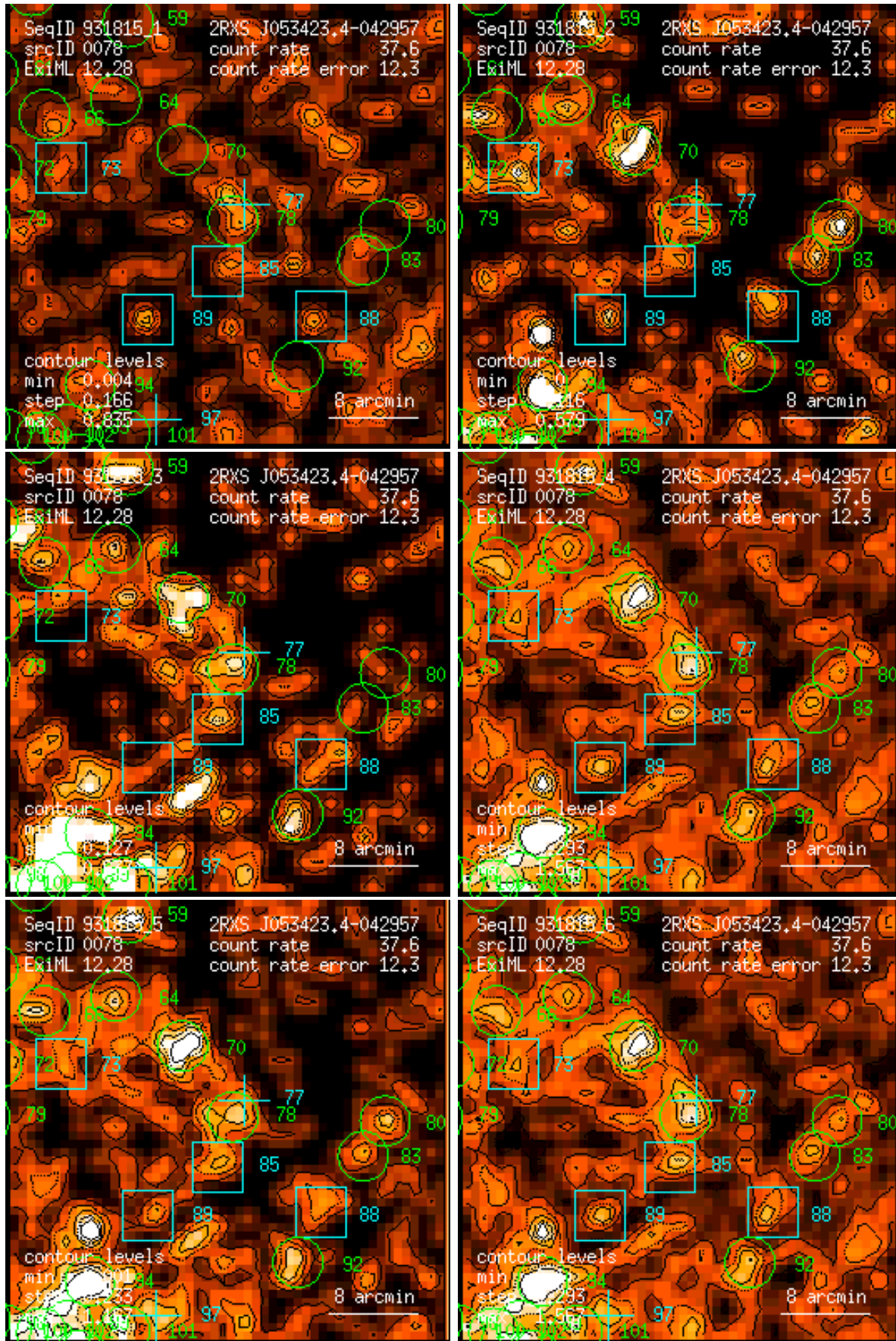
Figure 78: RASS 931815: detection 0078: band rate images, Gaussian filter: (1) PSPC channels 11 – 41, (2) 52 – 90, (3) 91 – 201, (4) 11 – 235, (5) 52 – 201, (6) 11 – 201. Broad band rates in counts/ks. Band rate contour levels in counts/ks/arcmin 2 .
