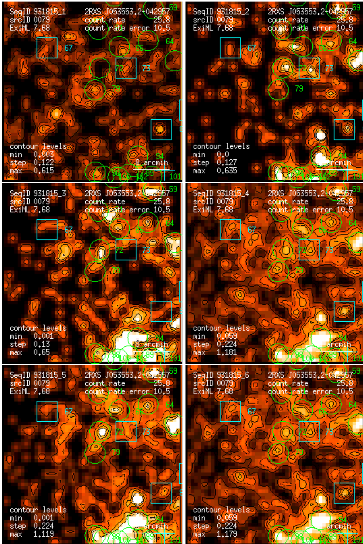
Figure 79: RASS 931815: detection 0079: band rate images, Gaussian filter: (1) PSPC channels 11 – 41, (2) 52 – 90, (3) 91 – 201, (4) 11 – 235, (5) 52 – 201, (6) 11 – 201. Broad band rates in counts/ks. Band rate contour levels in counts/ks/arcmin 2 .
