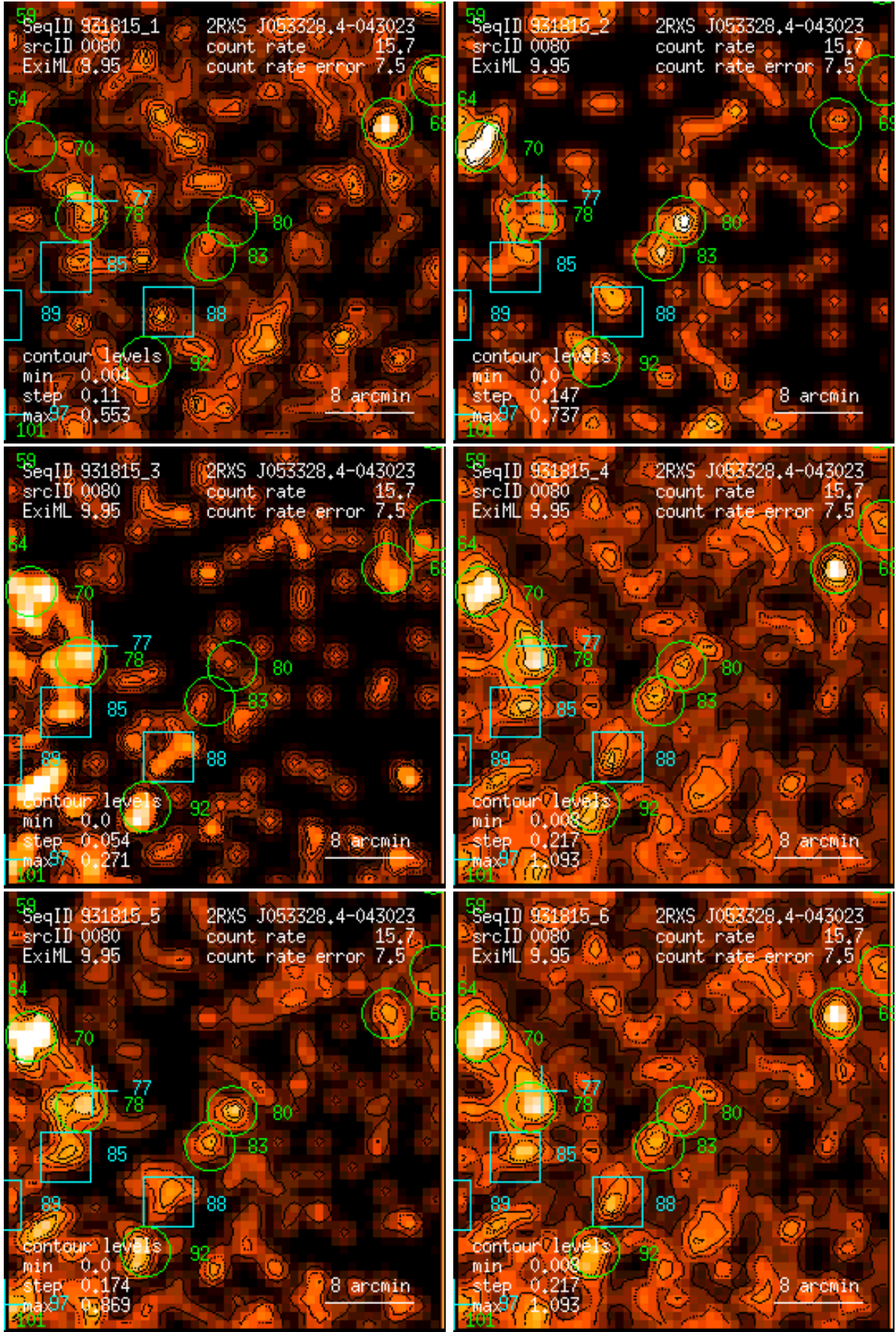
Figure 80: RASS 931815: detection 0080: band rate images, Gaussian filter: (1) PSPC channels 11 – 41, (2) 52 – 90, (3) 91 – 201, (4) 11 – 235, (5) 52 – 201, (6) 11 – 201. Broad band rates in counts/ks. Band rate contour levels in counts/ks/arcmin 2 .
