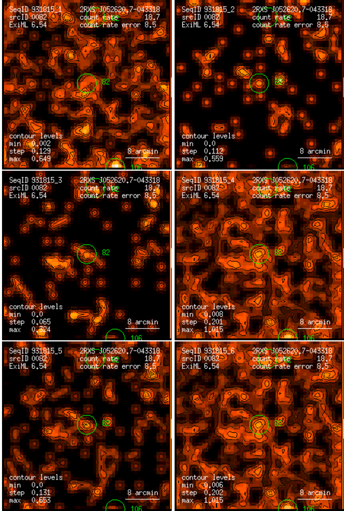
Figure 82: RASS 931815: detection 0082: band rate images, Gaussian filter: (1) PSPC channels 11 – 41, (2) 52 – 90, (3) 91 – 201, (4) 11 – 235, (5) 52 – 201, (6) 11 – 201. Broad band rates in counts/ks. Band rate contour levels in counts/ks/arcmin 2 .
