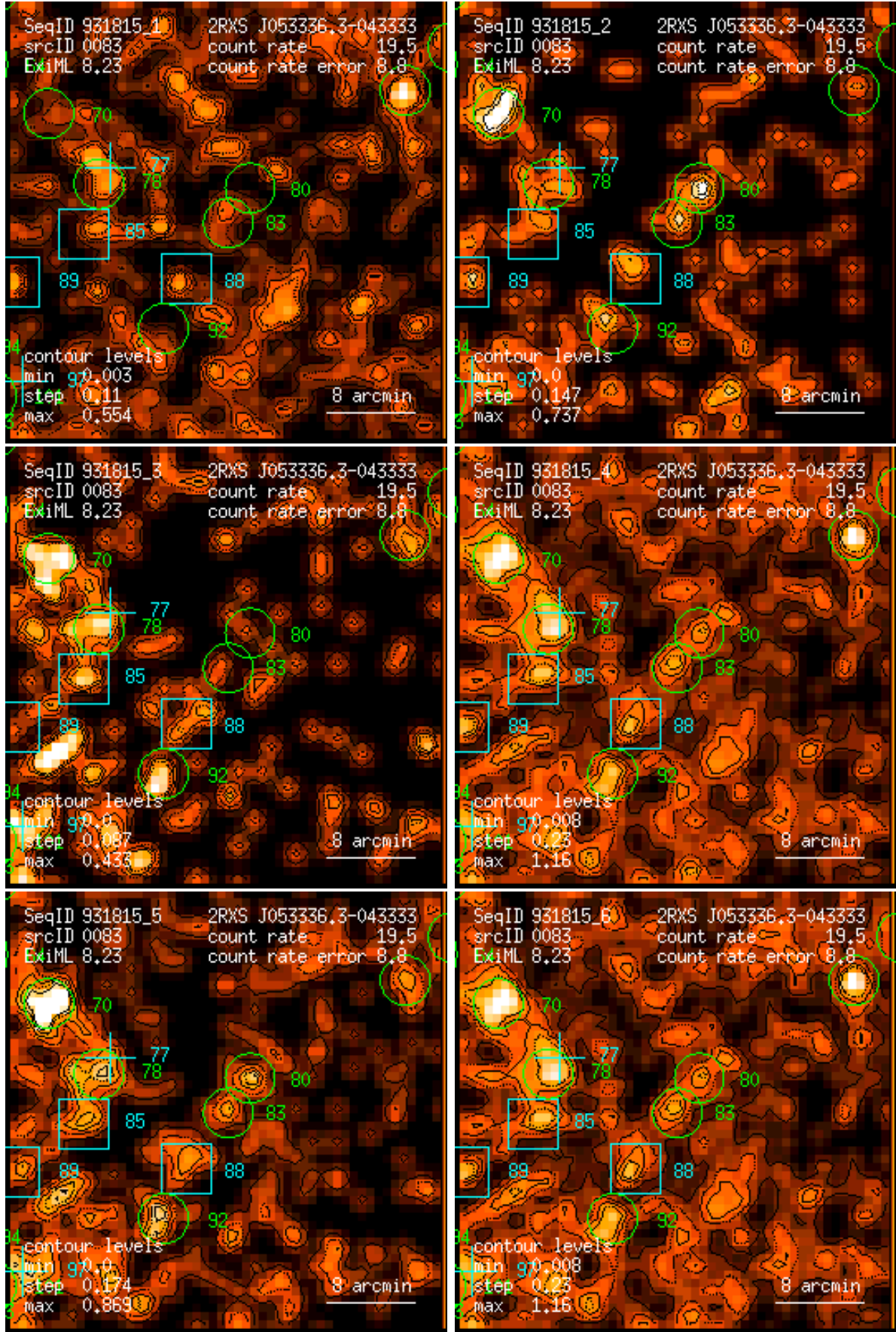
Figure 83: RASS 931815: detection 0083: band rate images, Gaussian filter: (1) PSPC channels 11 – 41, (2) 52 – 90, (3) 91 – 201, (4) 11 – 235, (5) 52 – 201, (6) 11 – 201. Broad band rates in counts/ks. Band rate contour levels in counts/ks/arcmin 2 .
