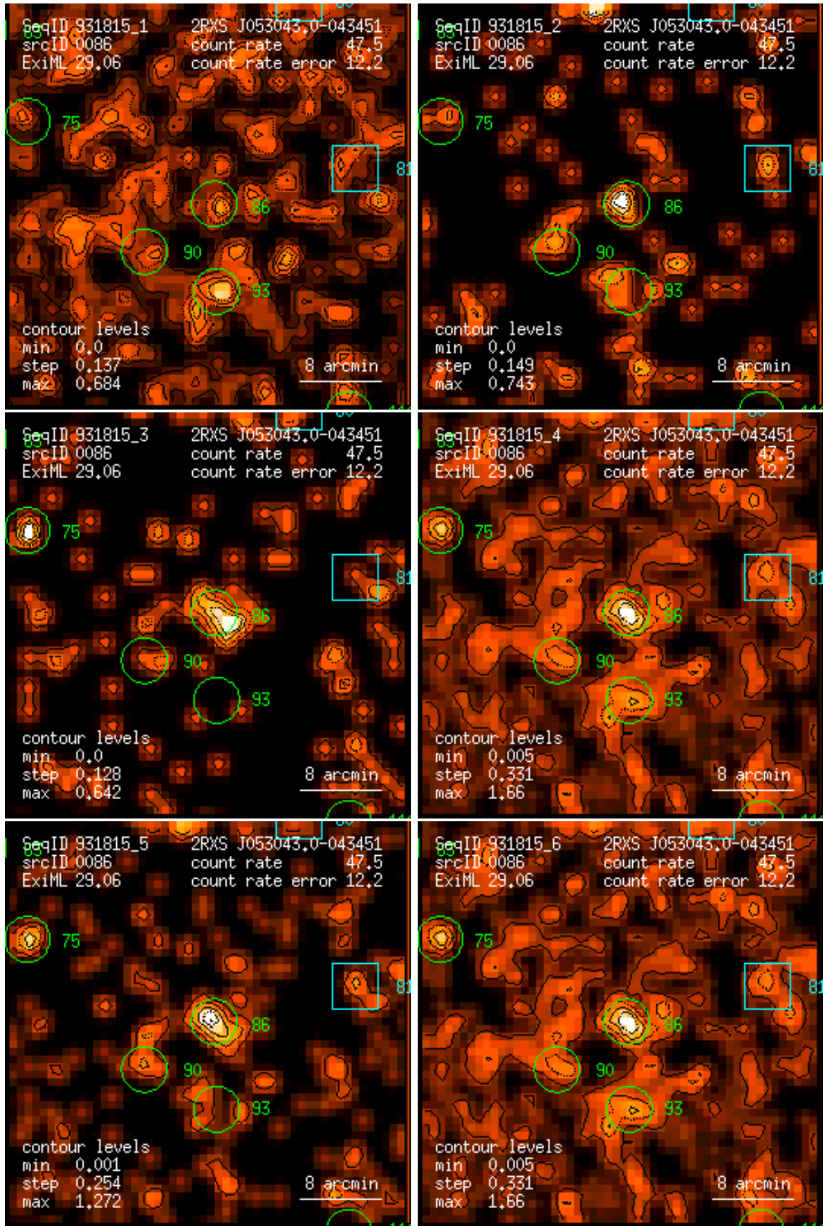
Figure 86: RASS 931815: detection 0086: band rate images, Gaussian filter: (1) PSPC channels 11 – 41, (2) 52 – 90, (3) 91 – 201, (4) 11 – 235, (5) 52 – 201, (6) 11 – 201. Broad band rates in counts/ks. Band rate contour levels in counts/ks/arcmin 2 .
