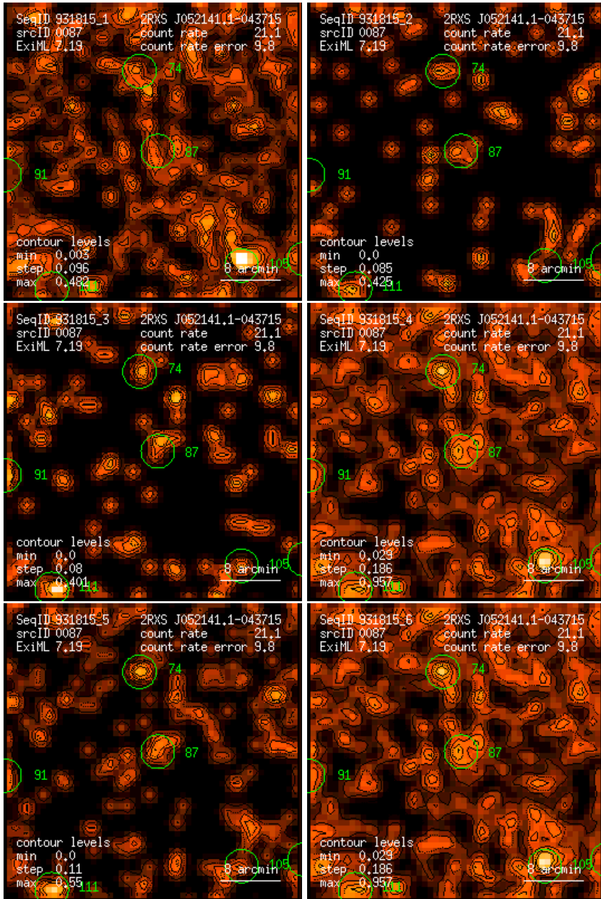
Figure 87: RASS 931815: detection 0087: band rate images, Gaussian filter: (1) PSPC channels 11 – 41, (2) 52 – 90, (3) 91 – 201, (4) 11 – 235, (5) 52 – 201, (6) 11 – 201. Broad band rates in counts/ks. Band rate contour levels in counts/ks/arcmin 2 .
