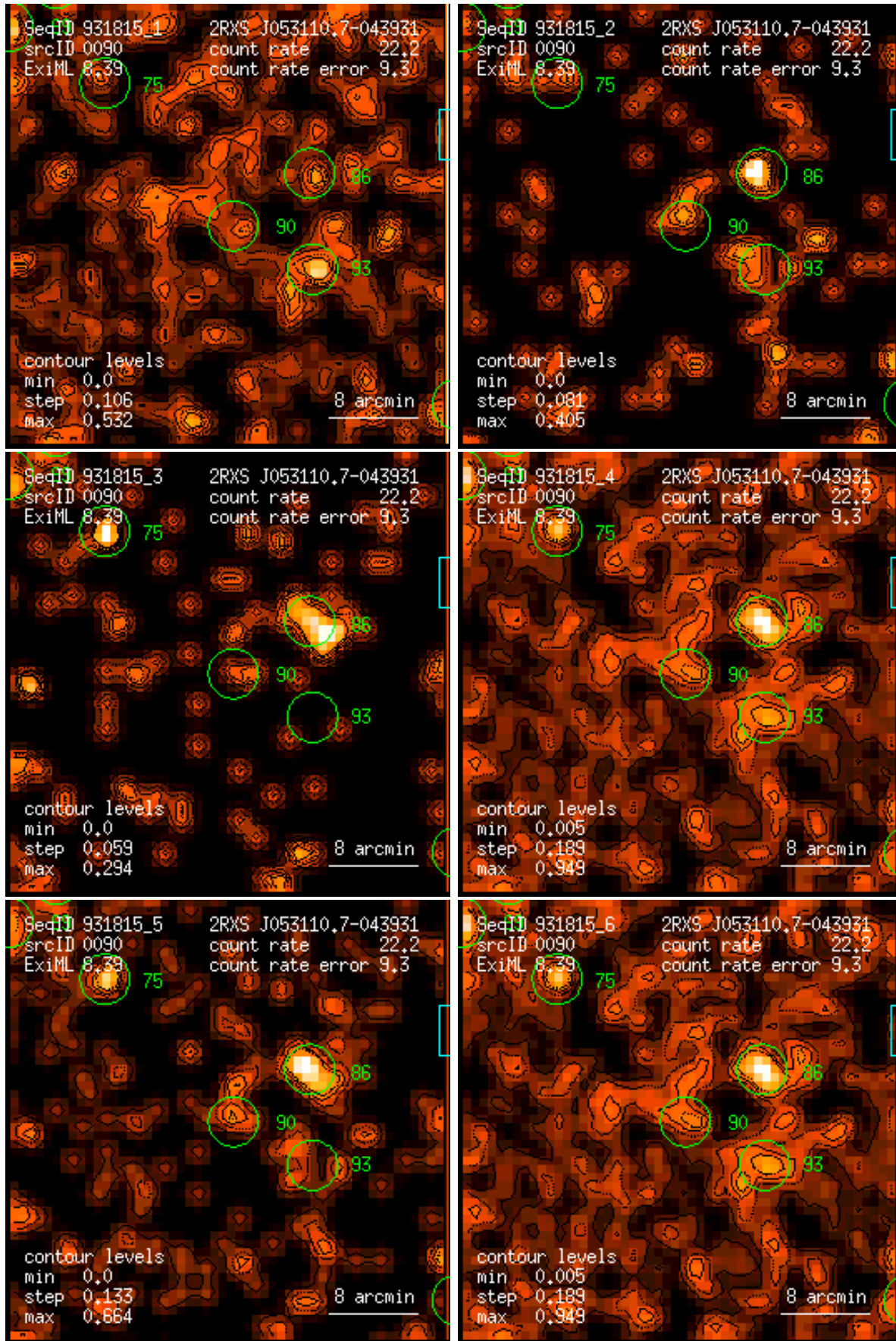
Figure 90: RASS 931815: detection 0090: band rate images, Gaussian filter: (1) PSPC channels 11 – 41, (2) 52 – 90, (3) 91 – 201, (4) 11 – 235, (5) 52 – 201, (6) 11 – 201. Broad band rates in counts/ks. Band rate contour levels in counts/ks/arcmin 2 .
