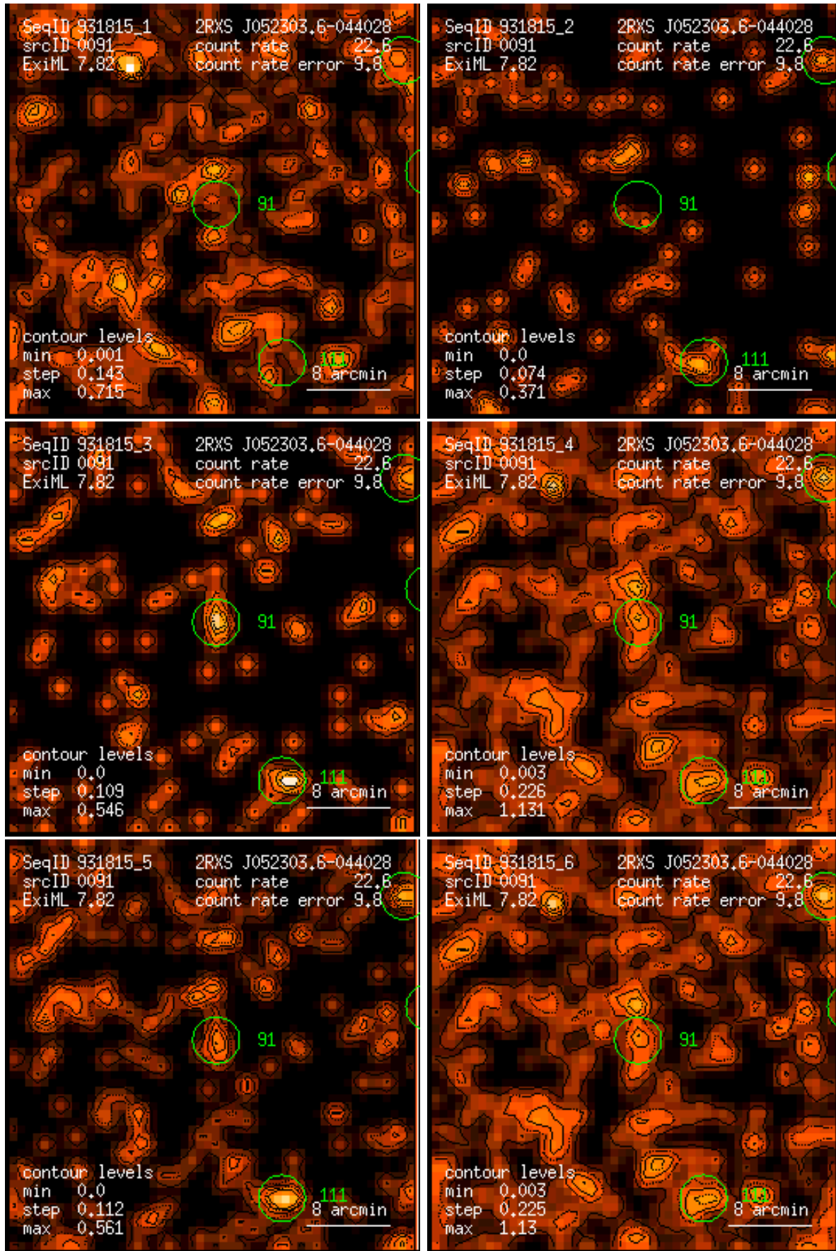
Figure 91: RASS 931815: detection 0091: band rate images, Gaussian filter: (1) PSPC channels 11 – 41, (2) 52 – 90, (3) 91 – 201, (4) 11 – 235, (5) 52 – 201, (6) 11 – 201. Broad band rates in counts/ks. Band rate contour levels in counts/ks/arcmin 2 .
