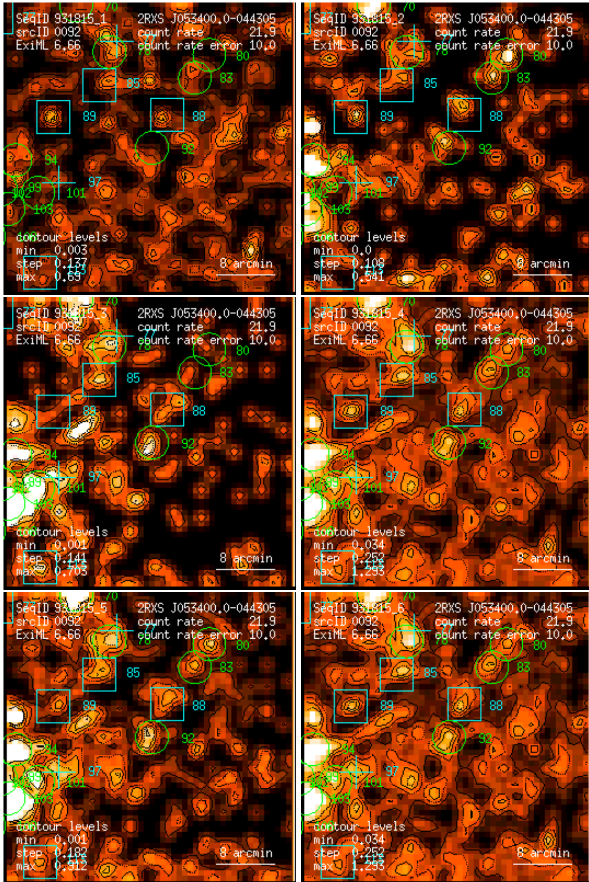
Figure 92: RASS 931815: detection 0092: band rate images, Gaussian filter: (1) PSPC channels 11 – 41, (2) 52 – 90, (3) 91 – 201, (4) 11 – 235, (5) 52 – 201, (6) 11 – 201. Broad band rates in counts/ks. Band rate contour levels in counts/ks/arcmin 2 .
