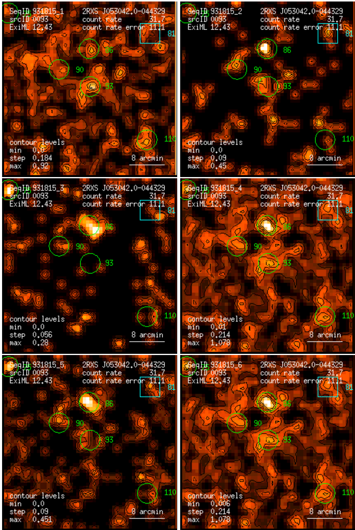
Figure 93: RASS 931815: detection 0093: band rate images, Gaussian filter: (1) PSPC channels 11 – 41, (2) 52 – 90, (3) 91 – 201, (4) 11 – 235, (5) 52 – 201, (6) 11 – 201. Broad band rates in counts/ks. Band rate contour levels in counts/ks/arcmin 2 .
