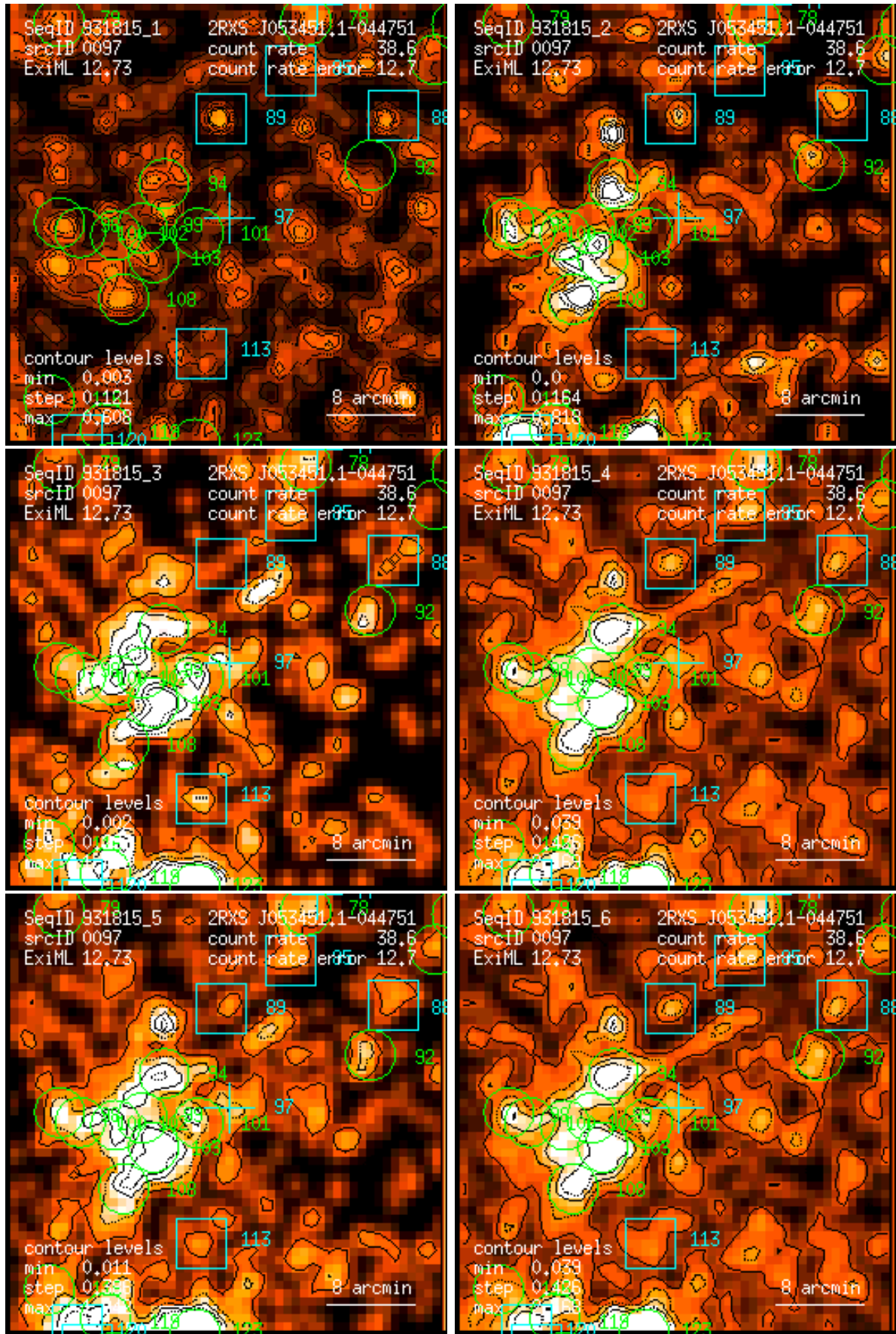
Figure 97: RASS 931815: detection 0097: band rate images, Gaussian filter: (1) PSPC channels 11 – 41, (2) 52 – 90, (3) 91 – 201, (4) 11 – 235, (5) 52 – 201, (6) 11 – 201. Broad band rates in counts/ks. Band rate contour levels in counts/ks/arcmin 2 .
