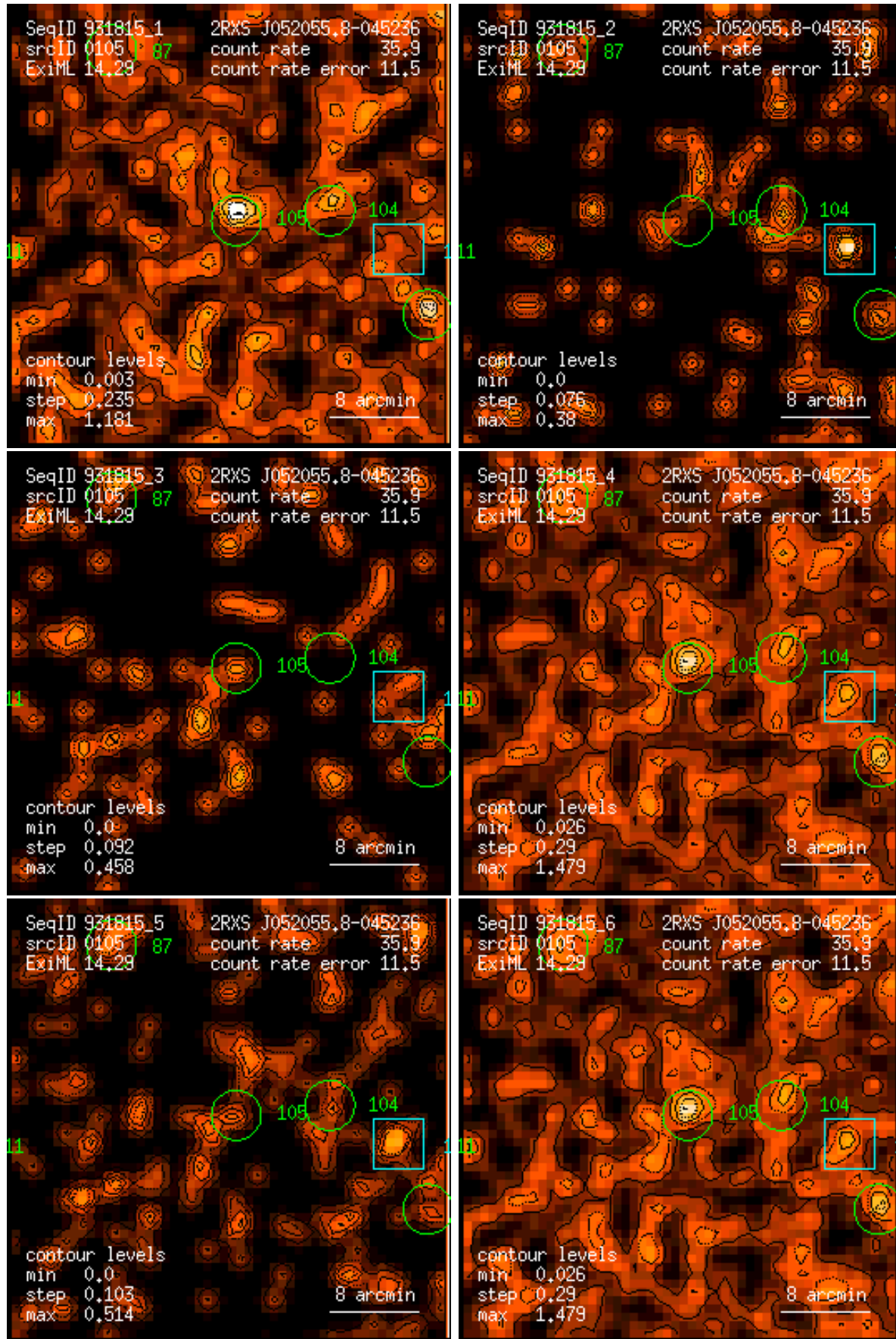
Figure 105: RASS 931815: detection 0105: band rate images, Gaussian filter: (1) PSPC channels 11 – 41, (2) 52 – 90, (3) 91 – 201, (4) 11 – 235, (5) 52 – 201, (6) 11 – 201. Broad band rates in counts/ks. Band rate contour levels in counts/ks/arcmin 2 .
