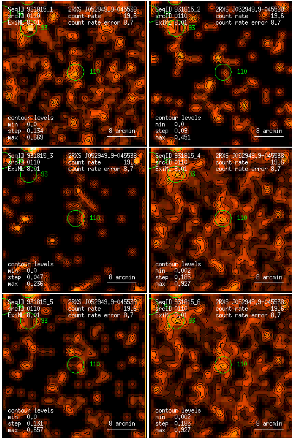
Figure 110: RASS 931815: detection 0110: band rate images, Gaussian filter: (1) PSPC channels 11 – 41, (2) 52 – 90, (3) 91 – 201, (4) 11 – 235, (5) 52 – 201, (6) 11 – 201. Broad band rates in counts/ks. Band rate contour levels in counts/ks/arcmin 2 .
