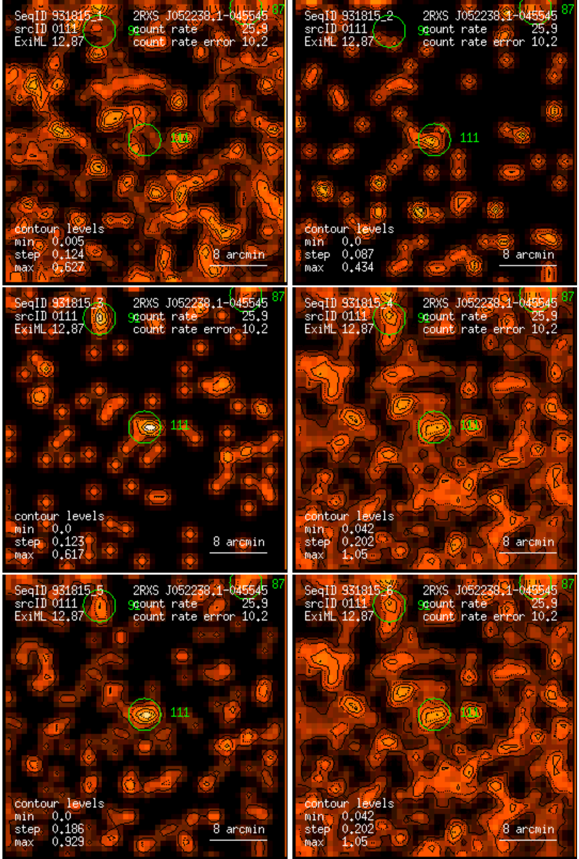
Figure 111: RASS 931815: detection 0111: band rate images, Gaussian filter: (1) PSPC channels 11 – 41, (2) 52 – 90, (3) 91 – 201, (4) 11 – 235, (5) 52 – 201, (6) 11 – 201. Broad band rates in counts/ks. Band rate contour levels in counts/ks/arcmin 2 .
