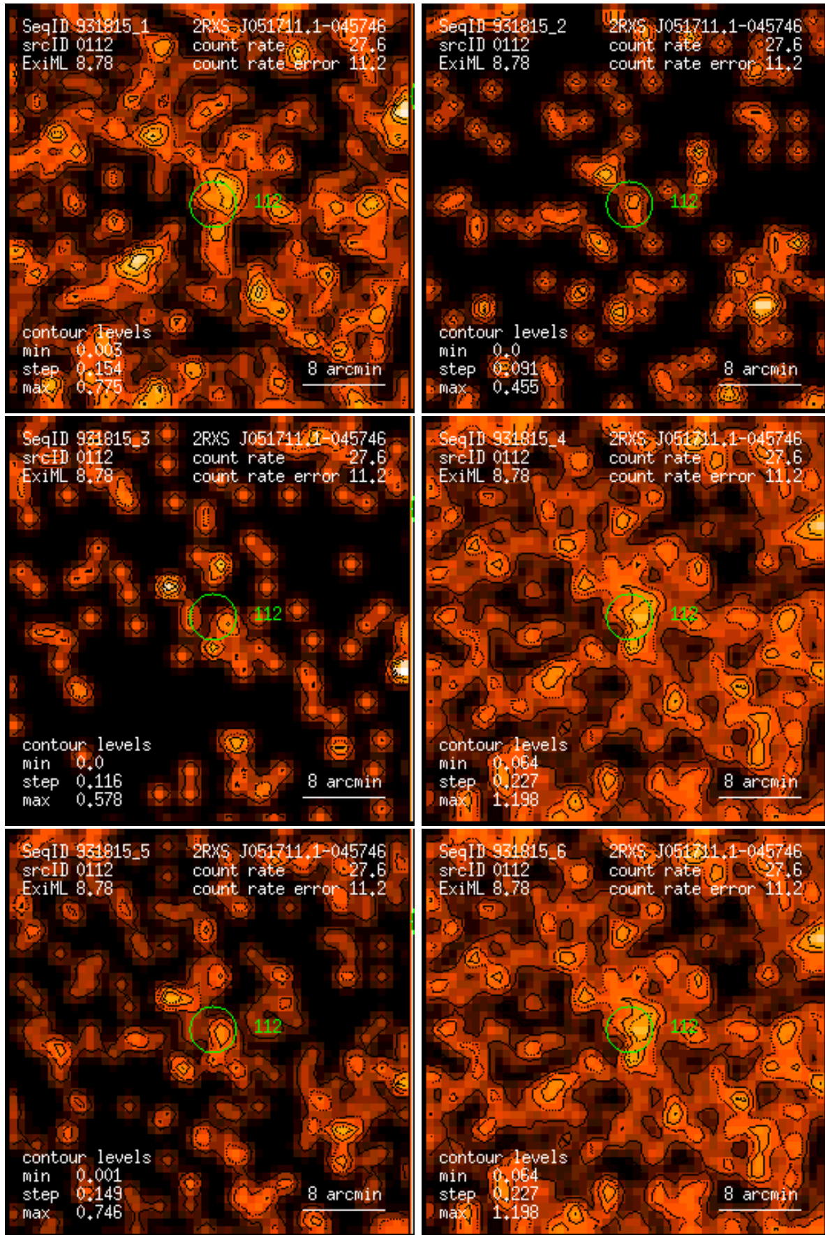
Figure 112: RASS 931815: detection 0112: band rate images, Gaussian filter: (1) PSPC channels 11 – 41, (2) 52 – 90, (3) 91 – 201, (4) 11 – 235, (5) 52 – 201, (6) 11 – 201. Broad band rates in counts/ks. Band rate contour levels in counts/ks/arcmin 2 .
