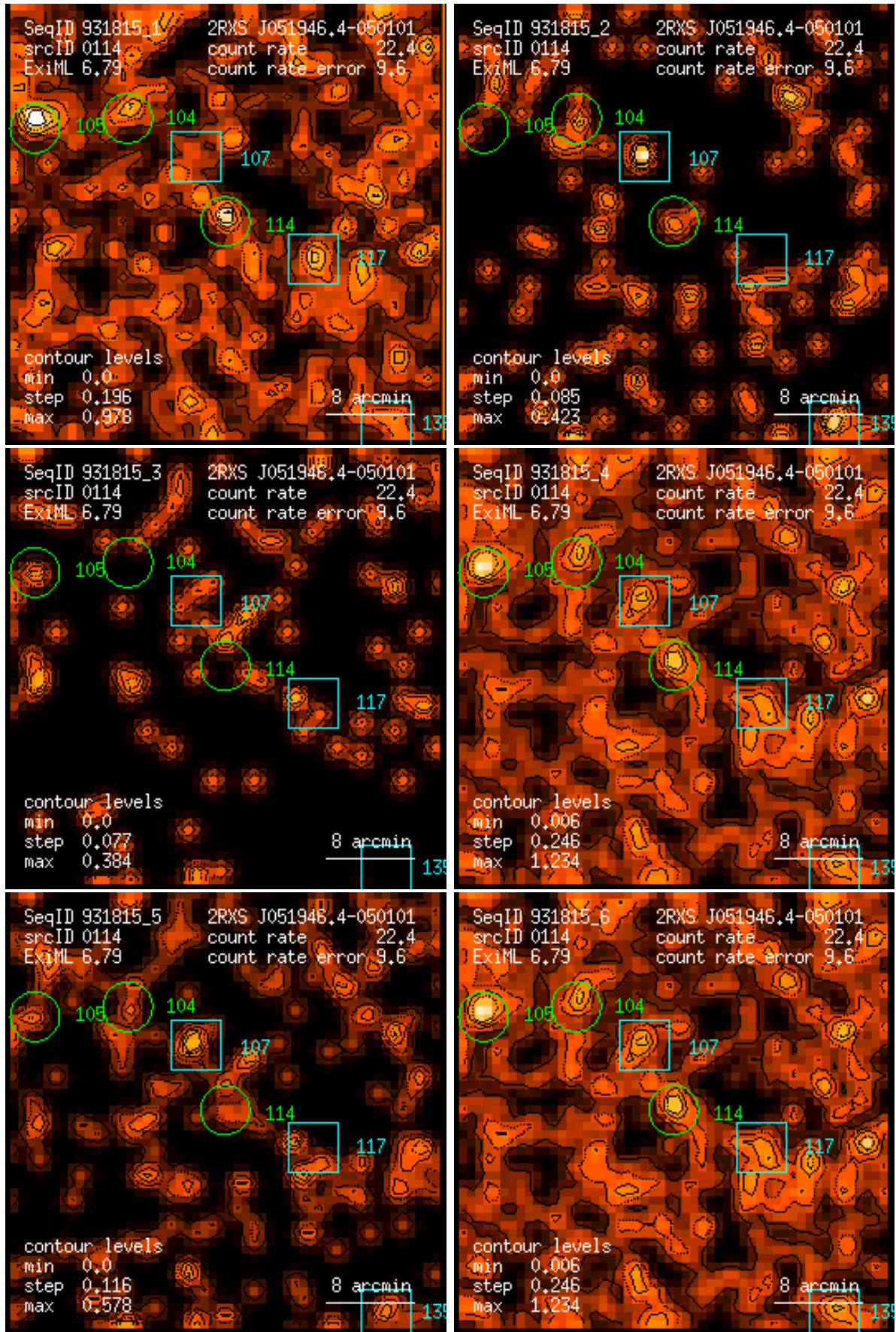
Figure 114: RASS 931815: detection 0114: band rate images, Gaussian filter: (1) PSPC channels 11 – 41, (2) 52 – 90, (3) 91 – 201, (4) 11 – 235, (5) 52 – 201, (6) 11 – 201. Broad band rates in counts/ks. Band rate contour levels in counts/ks/arcmin 2 .
