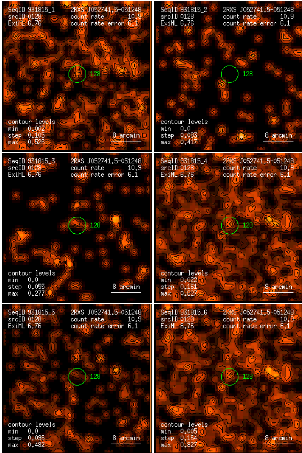
Figure 128: RASS 931815: detection 0128: band rate images, Gaussian filter: (1) PSPC channels 11 – 41, (2) 52 – 90, (3) 91 – 201, (4) 11 – 235, (5) 52 – 201, (6) 11 – 201. Broad band rates in counts/ks. Band rate contour levels in counts/ks/arcmin 2 .
