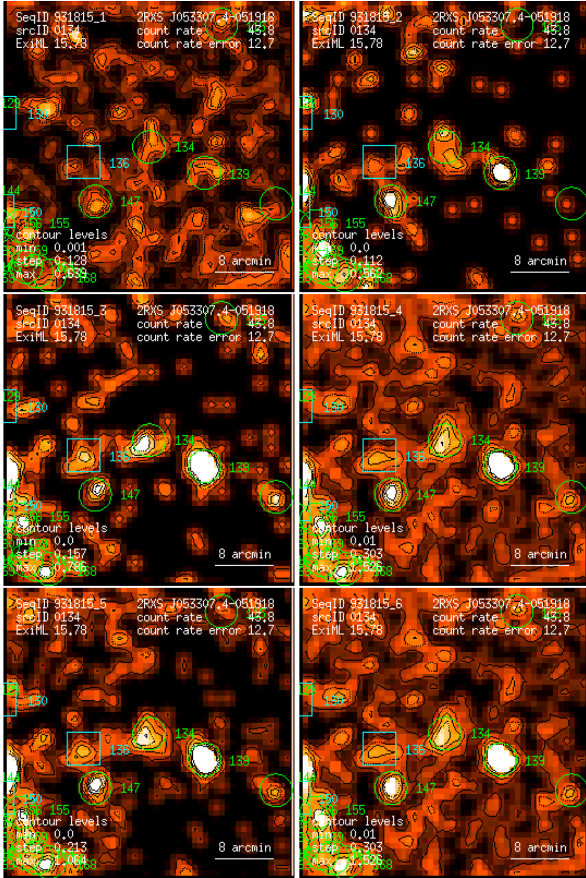
Figure 134: RASS 931815: detection 0134: band rate images, Gaussian filter: (1) PSPC channels 11 – 41, (2) 52 – 90, (3) 91 – 201, (4) 11 – 235, (5) 52 – 201, (6) 11 – 201. Broad band rates in counts/ks. Band rate contour levels in counts/ks/arcmin 2 .
