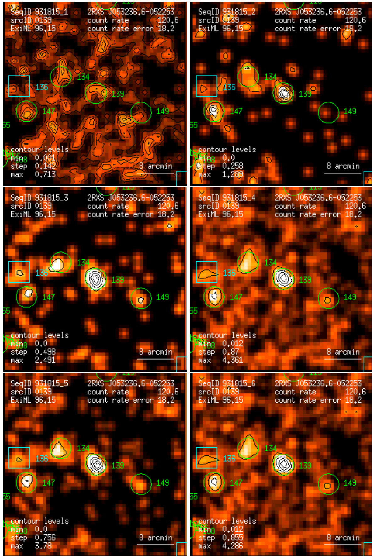
Figure 139: RASS 931815: detection 0139: band rate images, Gaussian filter: (1) PSPC channels 11 – 41, (2) 52 – 90, (3) 91 – 201, (4) 11 – 235, (5) 52 – 201, (6) 11 – 201. Broad band rates in counts/ks. Band rate contour levels in counts/ks/arcmin 2 .
