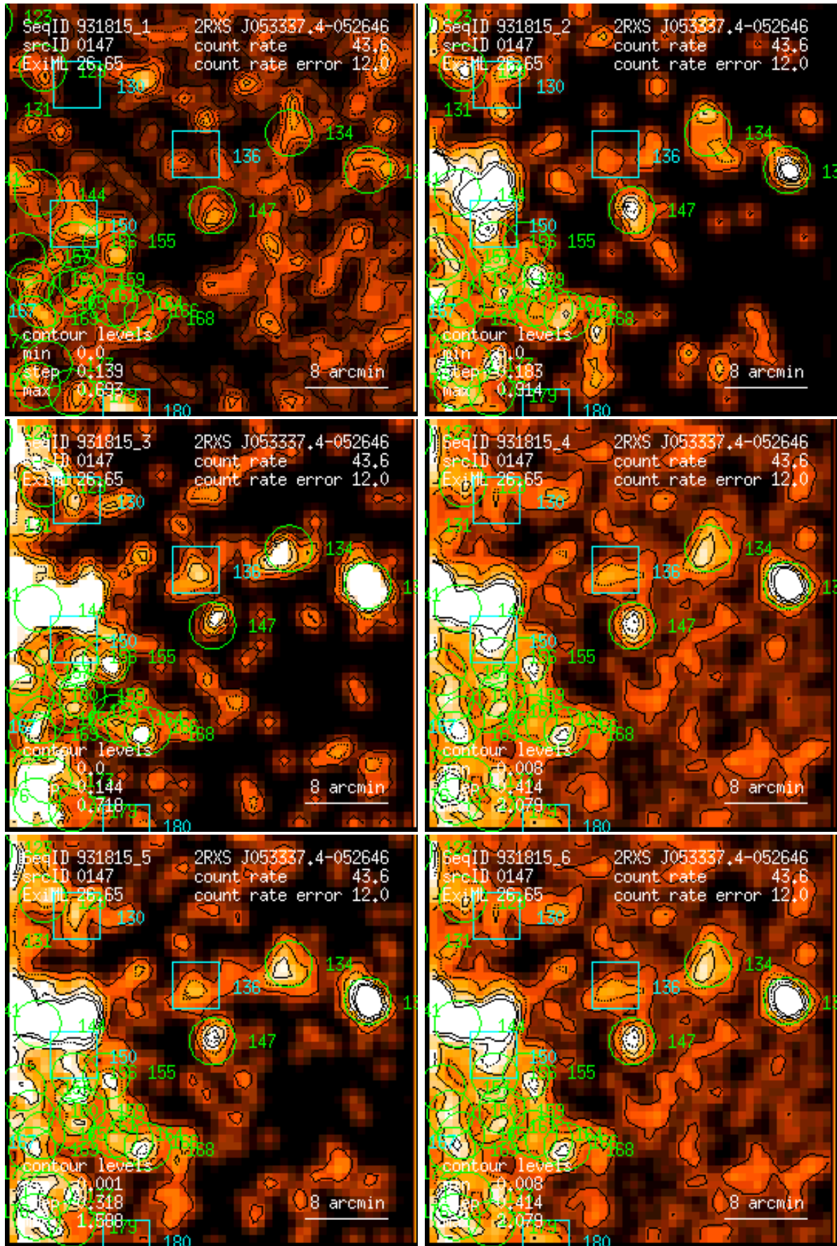
Figure 147: RASS 931815: detection 0147: band rate images, Gaussian filter: (1) PSPC channels 11 – 41, (2) 52 – 90, (3) 91 – 201, (4) 11 – 235, (5) 52 – 201, (6) 11 – 201. Broad band rates in counts/ks. Band rate contour levels in counts/ks/arcmin 2 .
