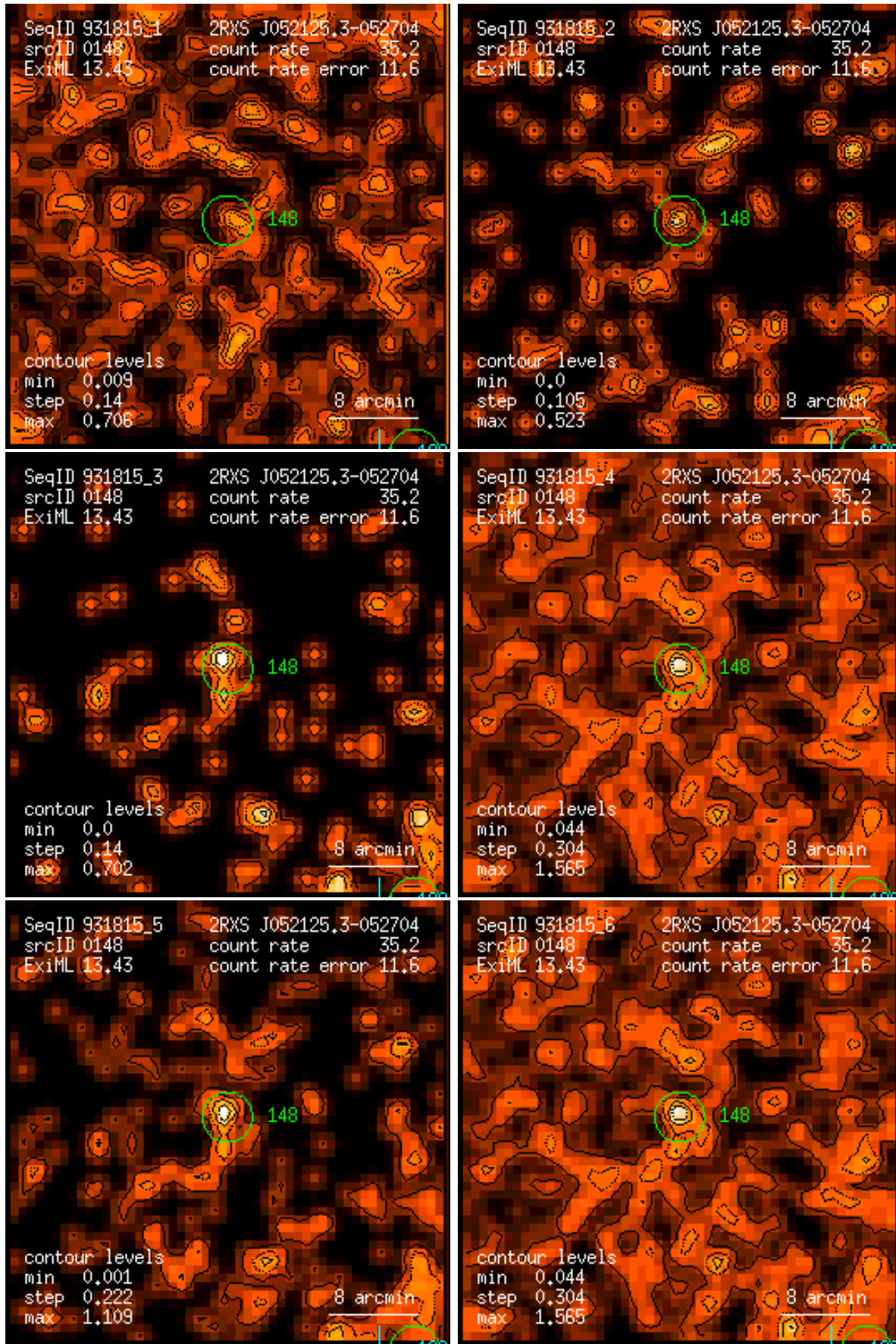
Figure 148: RASS 931815: detection 0148: band rate images, Gaussian filter: (1) PSPC channels 11 – 41, (2) 52 – 90, (3) 91 – 201, (4) 11 – 235, (5) 52 – 201, (6) 11 – 201. Broad band rates in counts/ks. Band rate contour levels in counts/ks/arcmin 2 .
