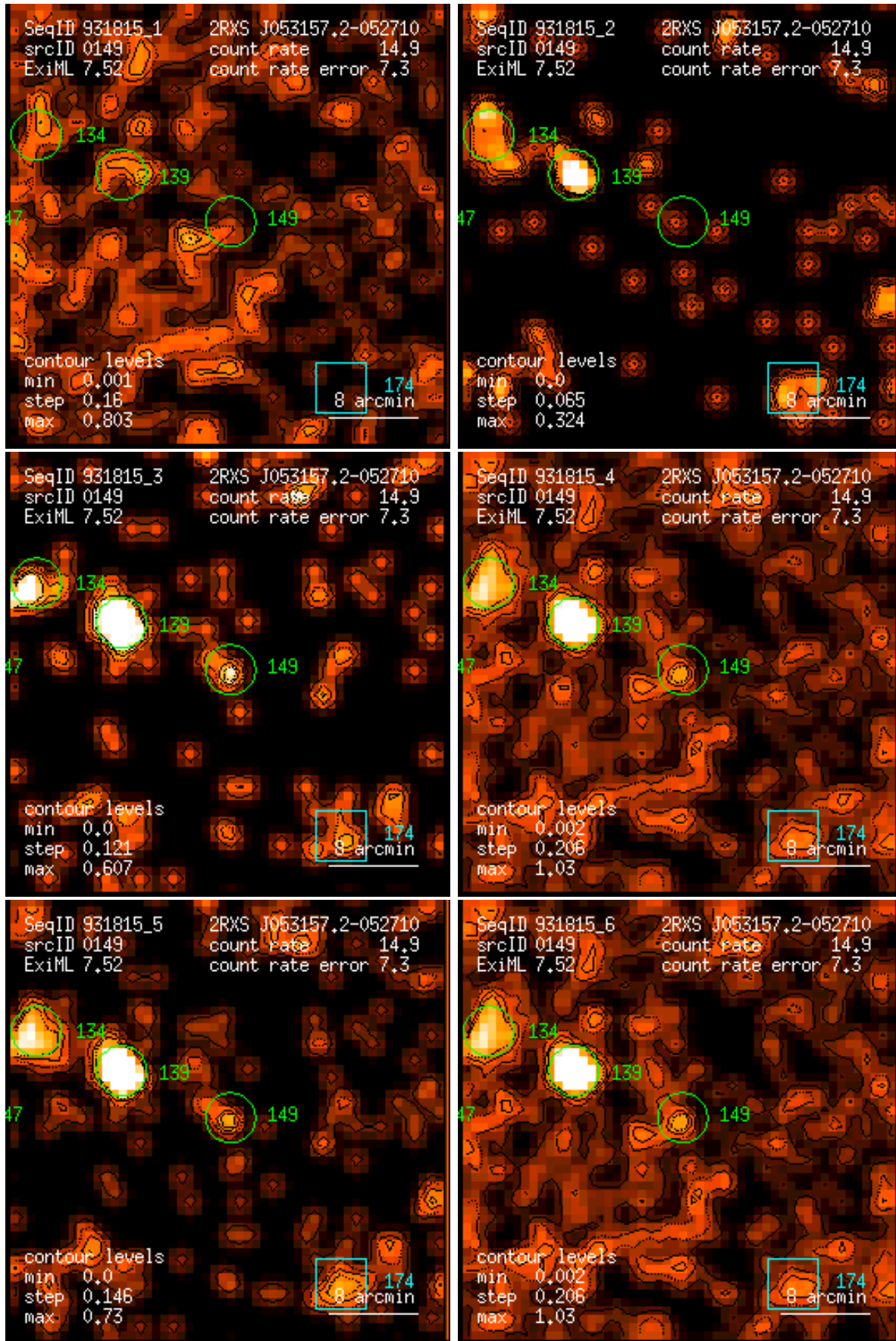
Figure 149: RASS 931815: detection 0149: band rate images, Gaussian filter: (1) PSPC channels 11 – 41, (2) 52 – 90, (3) 91 – 201, (4) 11 – 235, (5) 52 – 201, (6) 11 – 201. Broad band rates in counts/ks. Band rate contour levels in counts/ks/arcmin 2 .
