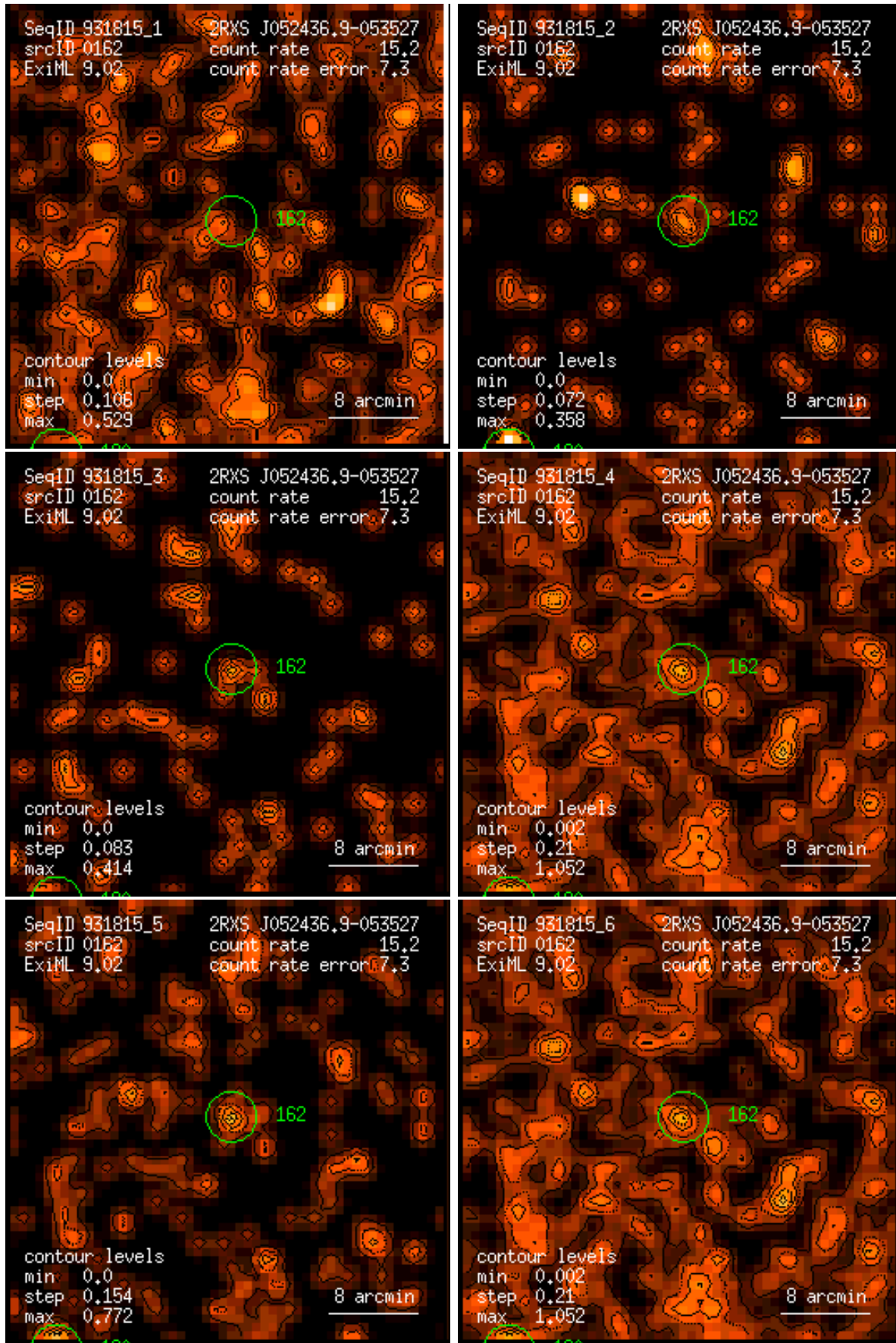
Figure 162: RASS 931815: detection 0162: band rate images, Gaussian filter: (1) PSPC channels 11 – 41, (2) 52 – 90, (3) 91 – 201, (4) 11 – 235, (5) 52 – 201, (6) 11 – 201. Broad band rates in counts/ks. Band rate contour levels in counts/ks/arcmin 2 .
