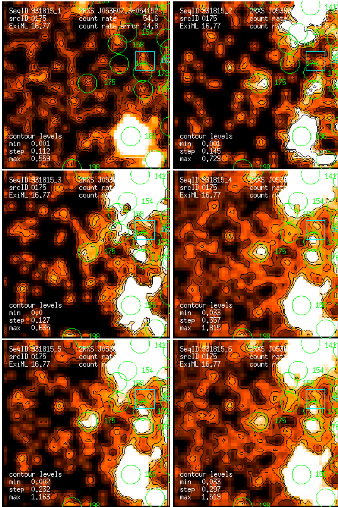
Figure 175: RASS 931815: detection 0175: band rate images, Gaussian filter: (1) PSPC channels 11 – 41, (2) 52 – 90, (3) 91 – 201, (4) 11 – 235, (5) 52 – 201, (6) 11 – 201. Broad band rates in counts/ks. Band rate contour levels in counts/ks/arcmin 2 .
