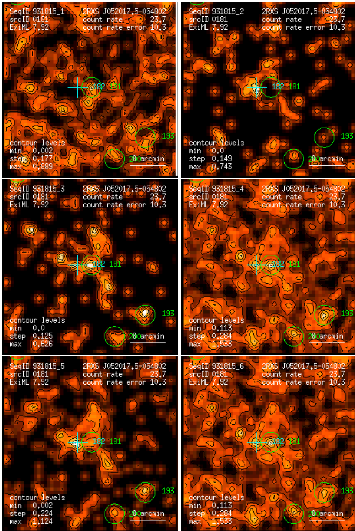
Figure 181: RASS 931815: detection 0181: band rate images, Gaussian filter: (1) PSPC channels 11 – 41, (2) 52 – 90, (3) 91 – 201, (4) 11 – 235, (5) 52 – 201, (6) 11 – 201. Broad band rates in counts/ks. Band rate contour levels in counts/ks/arcmin 2 .
