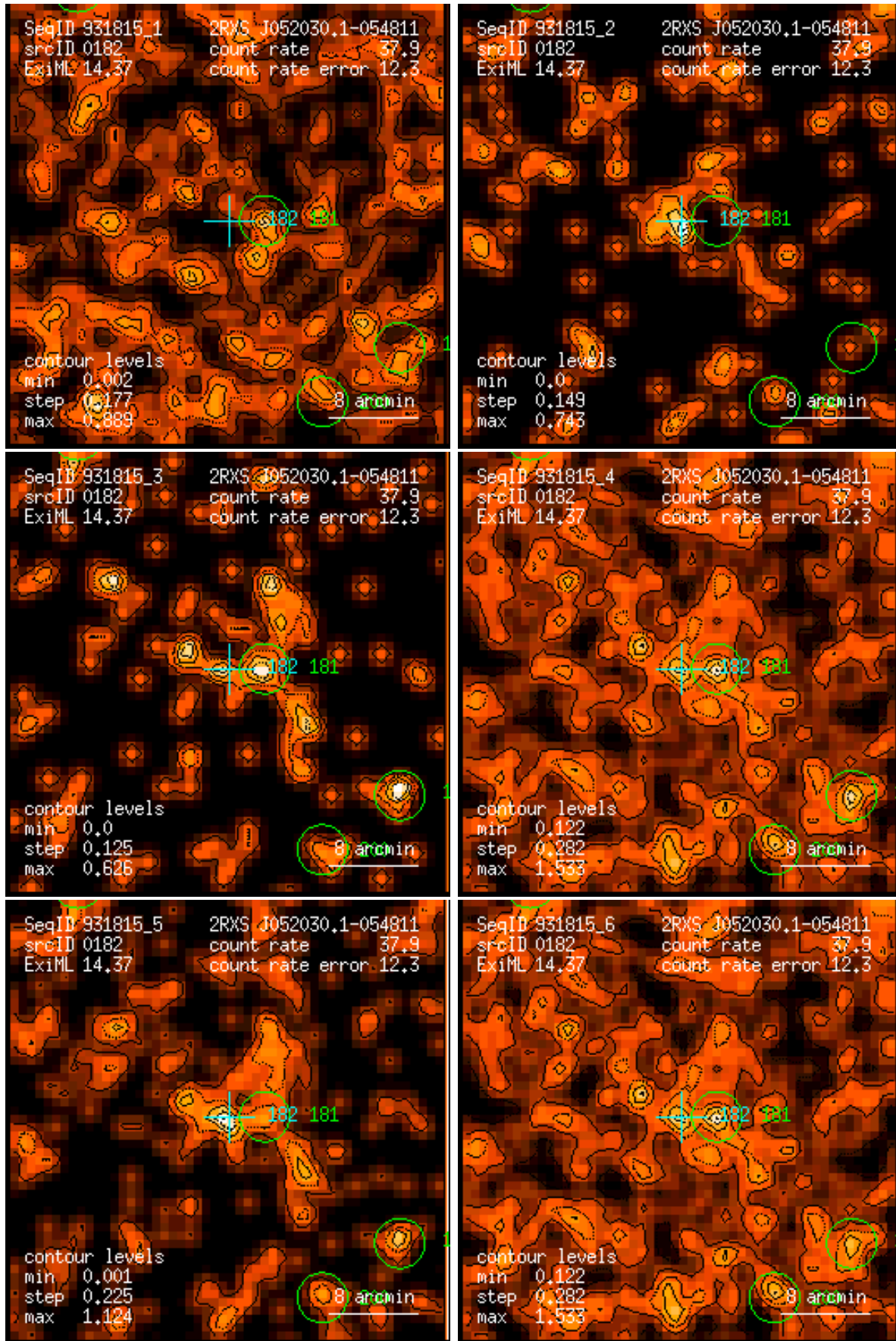
Figure 182: RASS 931815: detection 0182: band rate images, Gaussian filter: (1) PSPC channels 11 – 41, (2) 52 – 90, (3) 91 – 201, (4) 11 – 235, (5) 52 – 201, (6) 11 – 201. Broad band rates in counts/ks. Band rate contour levels in counts/ks/arcmin 2 .
