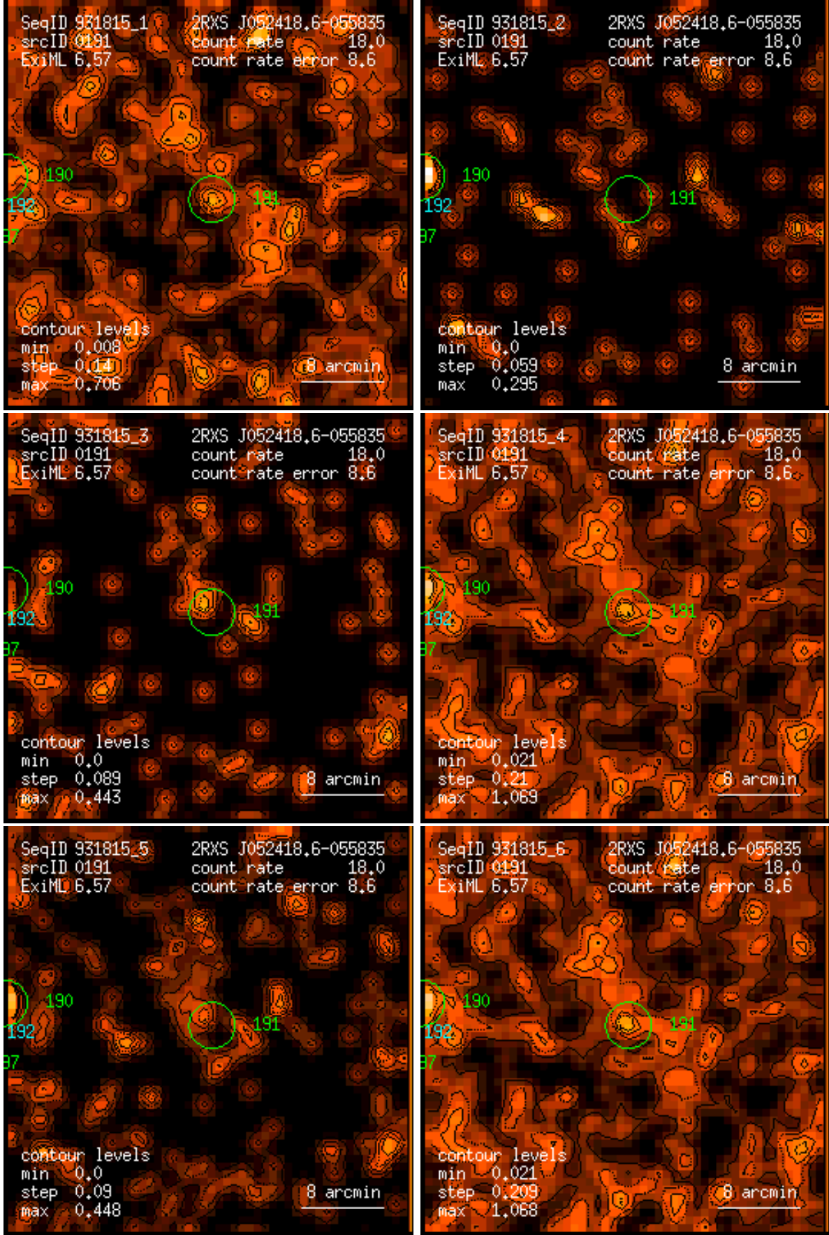
Figure 191: RASS 931815: detection 0191: band rate images, Gaussian filter: (1) PSPC channels 11 – 41, (2) 52 – 90, (3) 91 – 201, (4) 11 – 235, (5) 52 – 201, (6) 11 – 201. Broad band rates in counts/ks. Band rate contour levels in counts/ks/arcmin 2 .
