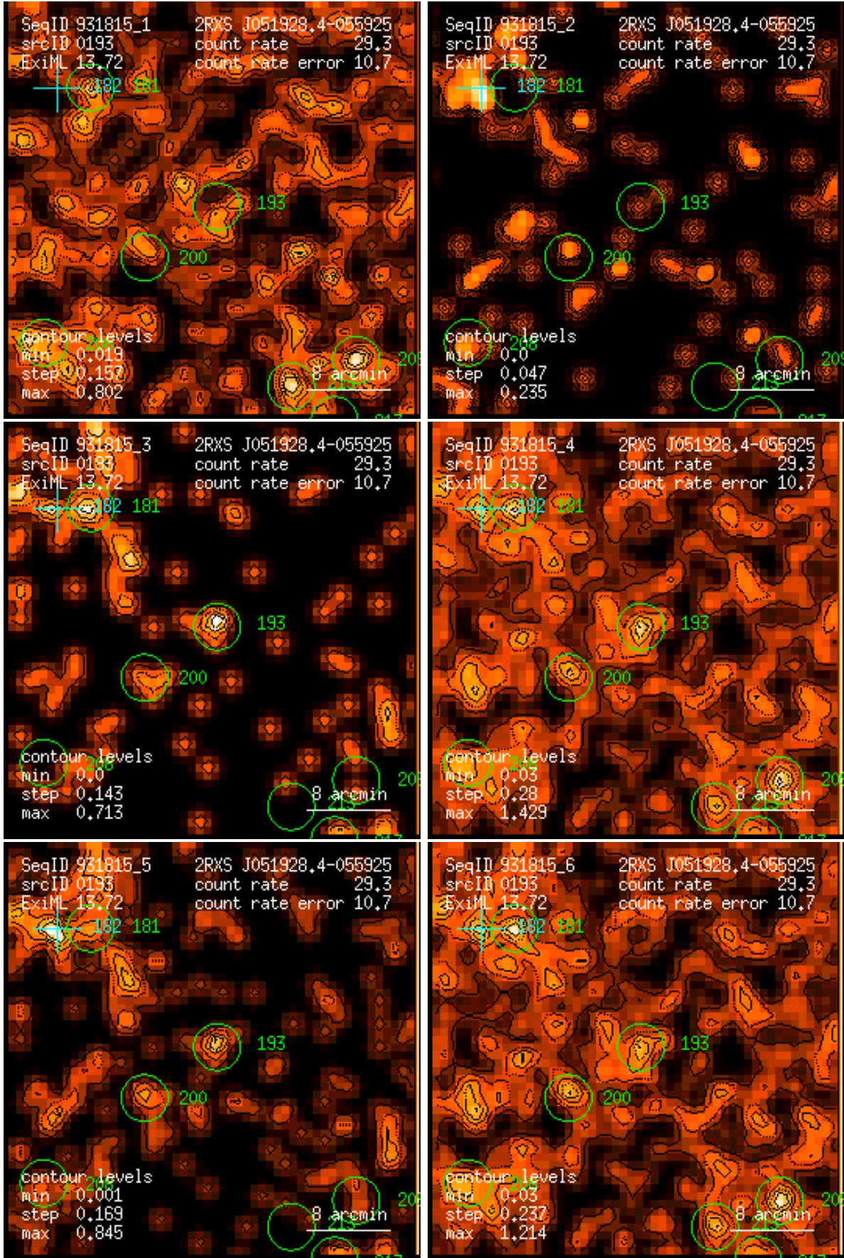
Figure 193: RASS 931815: detection 0193: band rate images, Gaussian filter: (1) PSPC channels 11 – 41, (2) 52 – 90, (3) 91 – 201, (4) 11 – 235, (5) 52 – 201, (6) 11 – 201. Broad band rates in counts/ks. Band rate contour levels in counts/ks/arcmin 2 .
