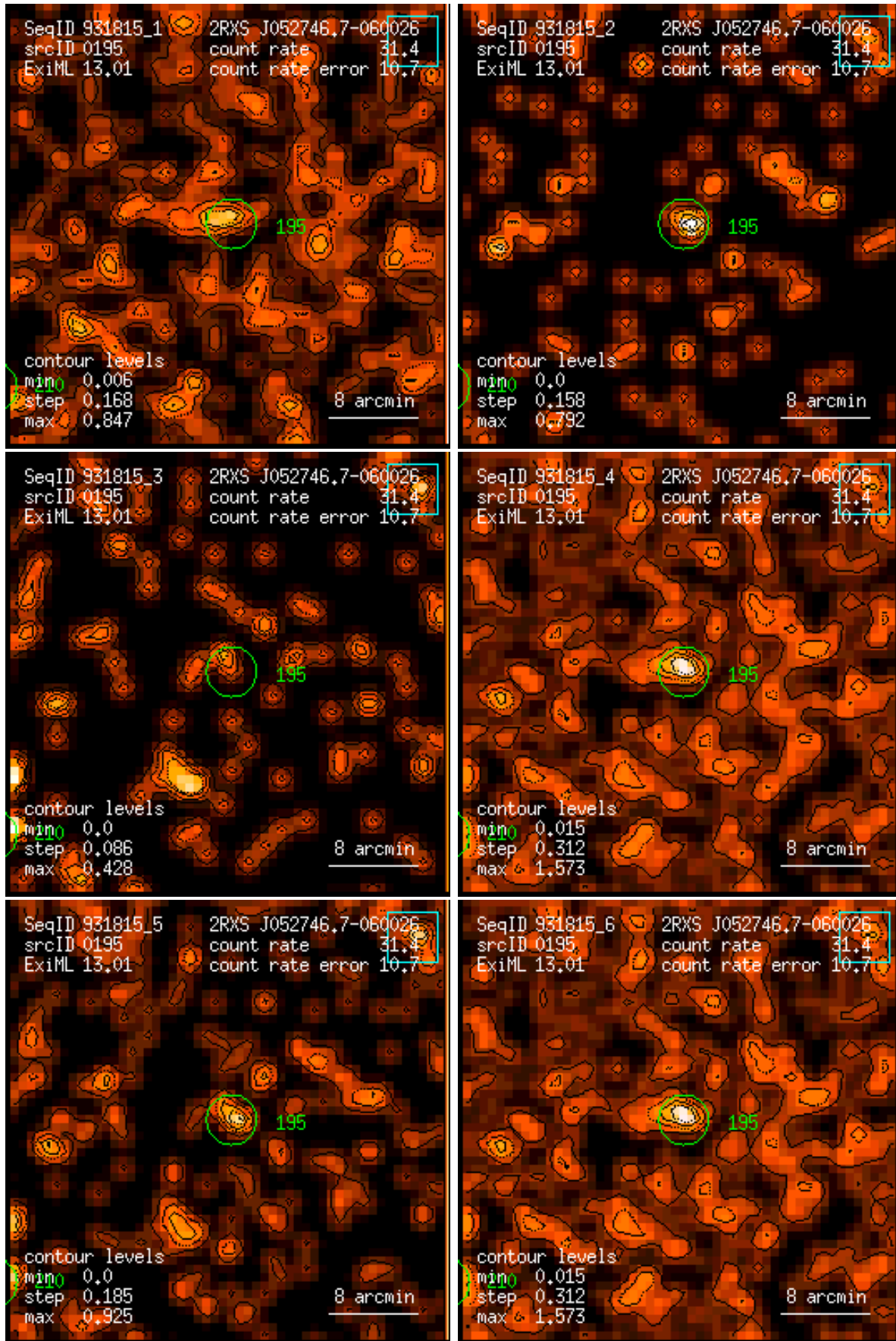
Figure 195: RASS 931815: detection 0195: band rate images, Gaussian filter: (1) PSPC channels 11 – 41, (2) 52 – 90, (3) 91 – 201, (4) 11 – 235, (5) 52 – 201, (6) 11 – 201. Broad band rates in counts/ks. Band rate contour levels in counts/ks/arcmin 2 .
