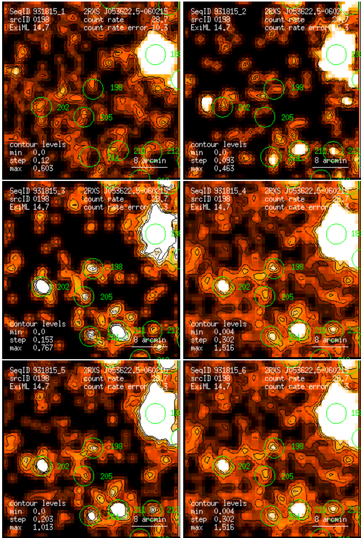
Figure 198: RASS 931815: detection 0198: band rate images, Gaussian filter: (1) PSPC channels 11 – 41, (2) 52 – 90, (3) 91 – 201, (4) 11 – 235, (5) 52 – 201, (6) 11 – 201. Broad band rates in counts/ks. Band rate contour levels in counts/ks/arcmin 2 .
