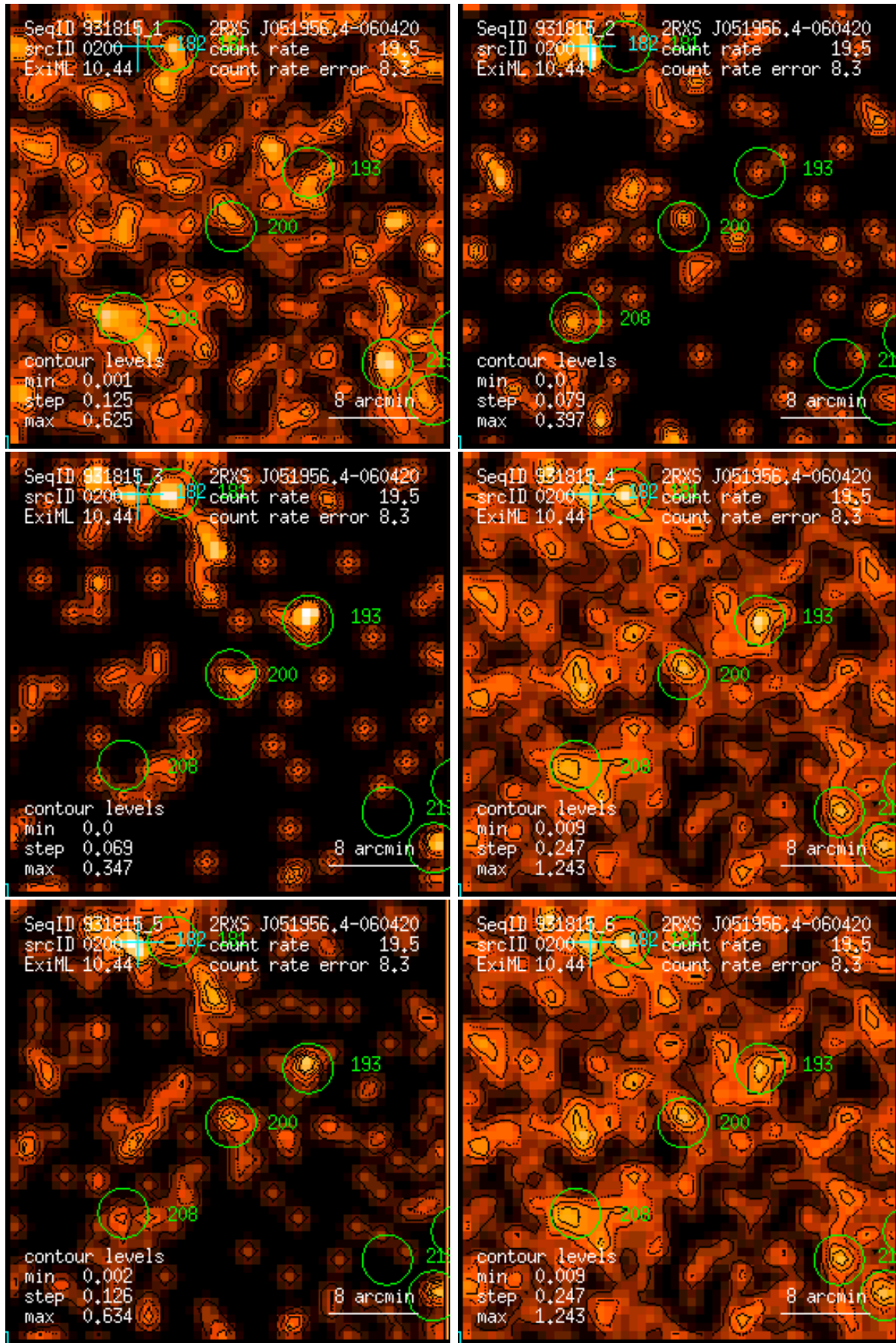
Figure 200: RASS 931815: detection 0200: band rate images, Gaussian filter: (1) PSPC channels 11 – 41, (2) 52 – 90, (3) 91 – 201, (4) 11 – 235, (5) 52 – 201, (6) 11 – 201. Broad band rates in counts/ks. Band rate contour levels in counts/ks/arcmin 2 .
