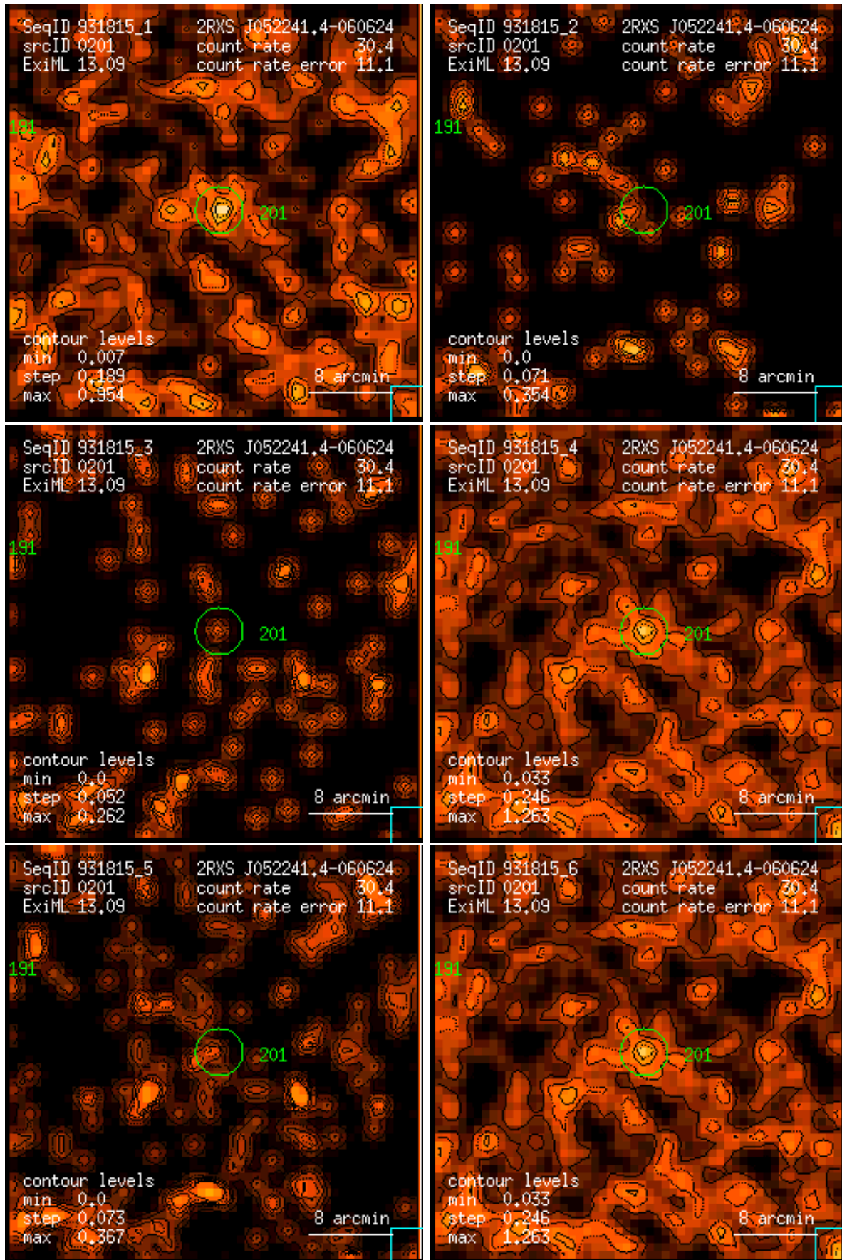
Figure 201: RASS 931815: detection 0201: band rate images, Gaussian filter: (1) PSPC channels 11 – 41, (2) 52 – 90, (3) 91 – 201, (4) 11 – 235, (5) 52 – 201, (6) 11 – 201. Broad band rates in counts/ks. Band rate contour levels in counts/ks/arcmin 2 .
