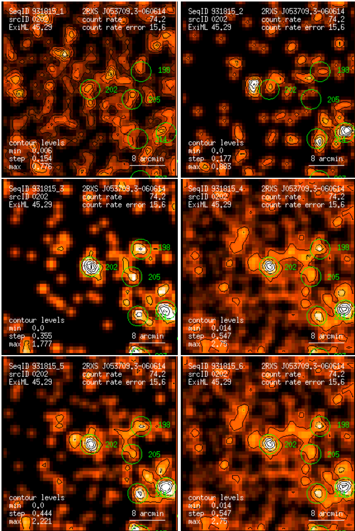
Figure 202: RASS 931815: detection 0202: band rate images, Gaussian filter: (1) PSPC channels 11 – 41, (2) 52 – 90, (3) 91 – 201, (4) 11 – 235, (5) 52 – 201, (6) 11 – 201. Broad band rates in counts/ks. Band rate contour levels in counts/ks/arcmin 2 .
