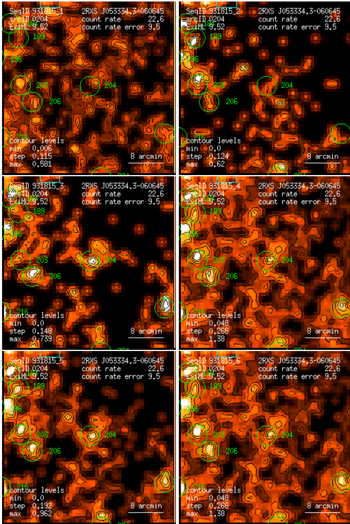
Figure 204: RASS 931815: detection 0204: band rate images, Gaussian filter: (1) PSPC channels 11 – 41, (2) 52 – 90, (3) 91 – 201, (4) 11 – 235, (5) 52 – 201, (6) 11 – 201. Broad band rates in counts/ks. Band rate contour levels in counts/ks/arcmin 2 .
