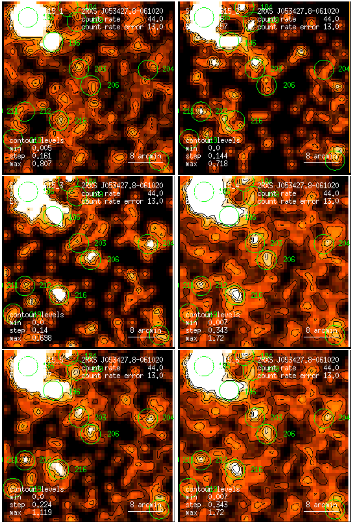
Figure 206: RASS 931815: detection 0206: band rate images, Gaussian filter: (1) PSPC channels 11 – 41, (2) 52 – 90, (3) 91 – 201, (4) 11 – 235, (5) 52 – 201, (6) 11 – 201. Broad band rates in counts/ks. Band rate contour levels in counts/ks/arcmin 2 .
