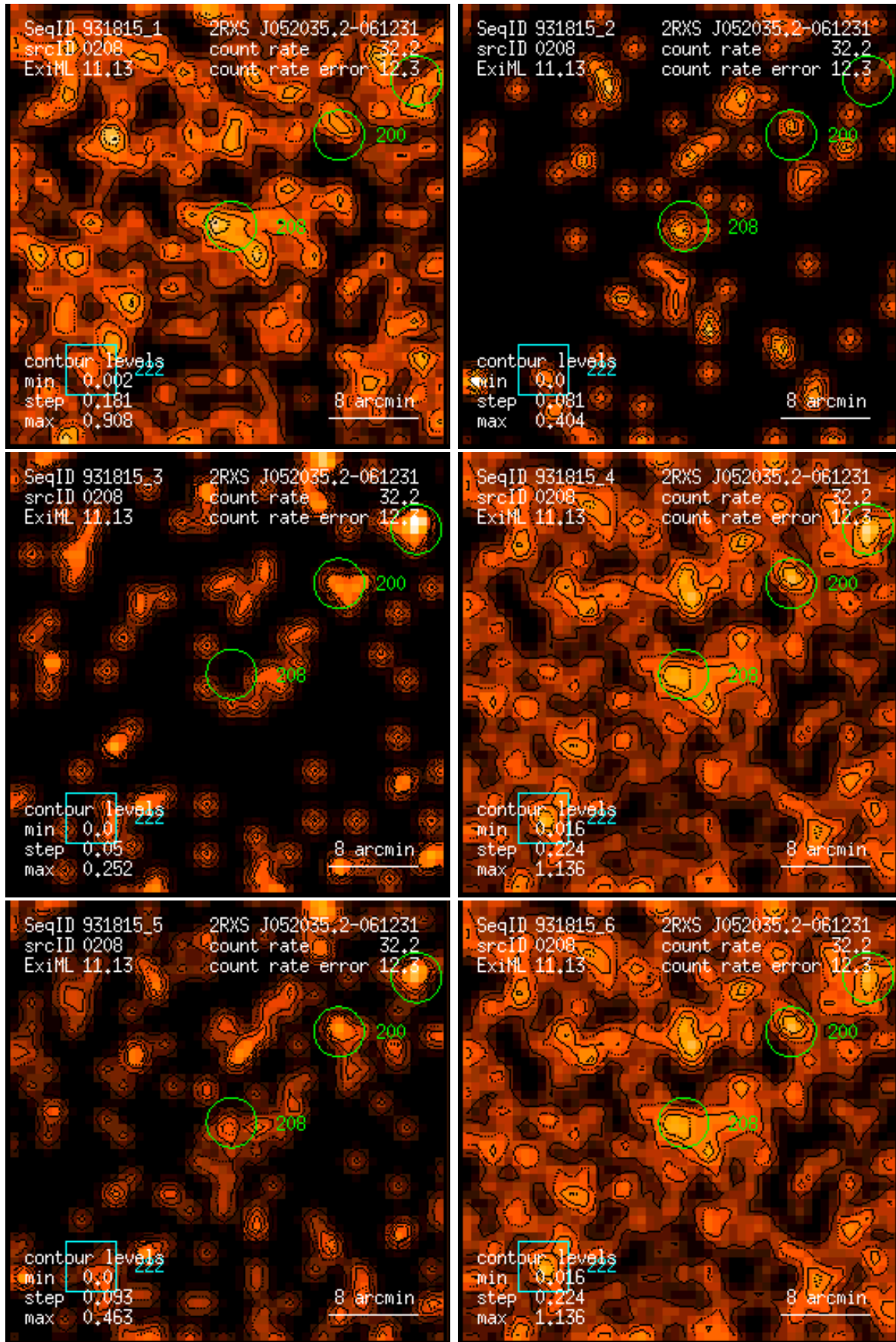
Figure 208: RASS 931815: detection 0208: band rate images, Gaussian filter: (1) PSPC channels 11 – 41, (2) 52 – 90, (3) 91 – 201, (4) 11 – 235, (5) 52 – 201, (6) 11 – 201. Broad band rates in counts/ks. Band rate contour levels in counts/ks/arcmin 2 .
