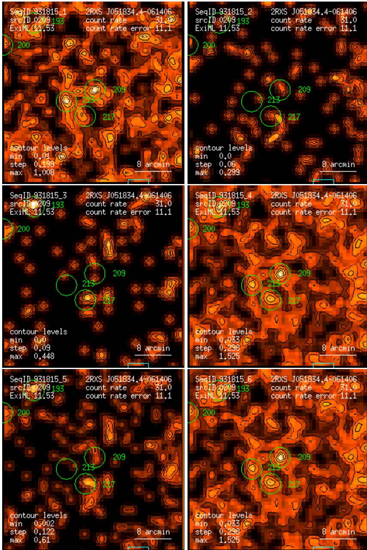
Figure 209: RASS 931815: detection 0209: band rate images, Gaussian filter: (1) PSPC channels 11 – 41, (2) 52 – 90, (3) 91 – 201, (4) 11 – 235, (5) 52 – 201, (6) 11 – 201. Broad band rates in counts/ks. Band rate contour levels in counts/ks/arcmin 2 .
