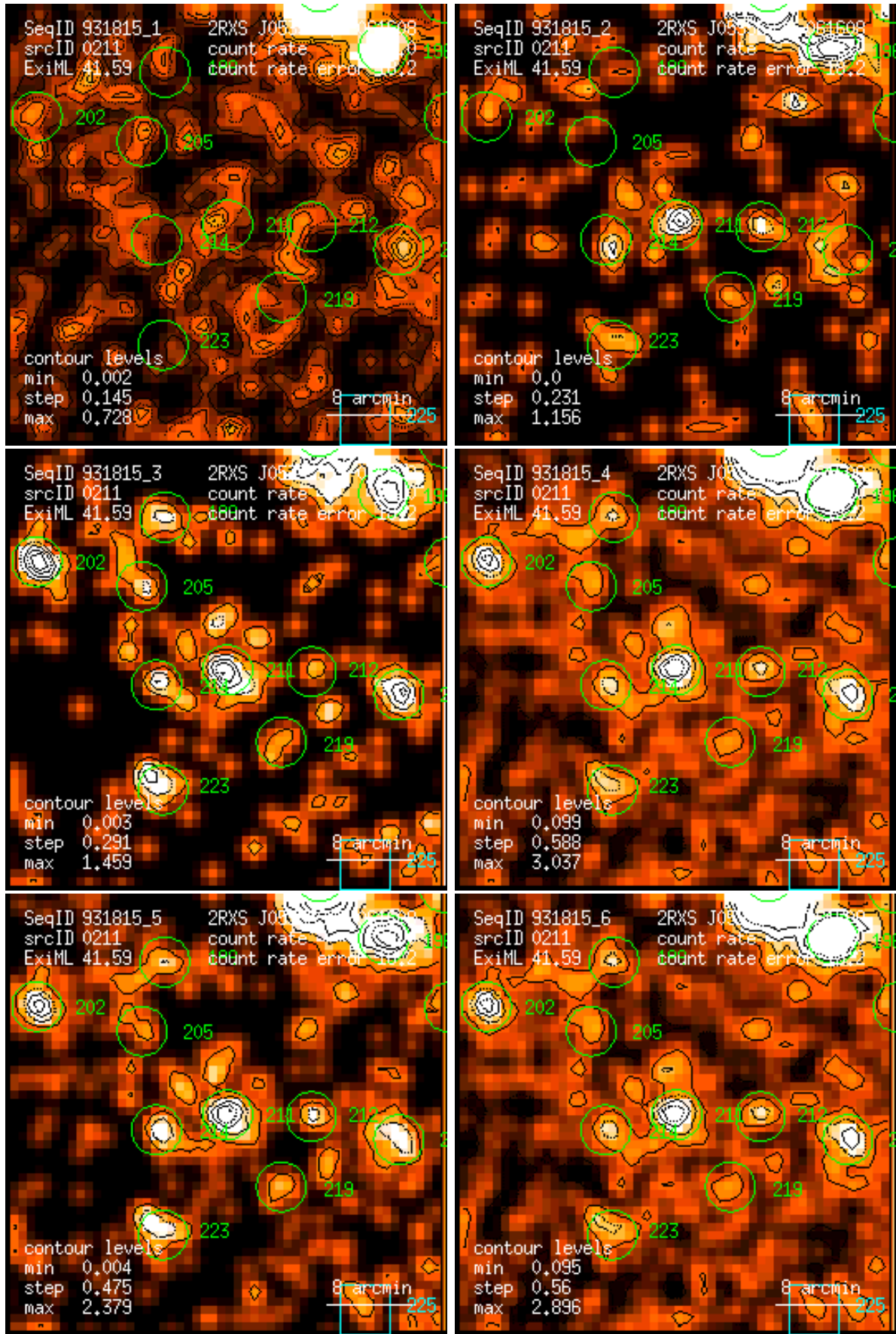
Figure 211: RASS 931815: detection 0211: band rate images, Gaussian filter: (1) PSPC channels 11 – 41, (2) 52 – 90, (3) 91 – 201, (4) 11 – 235, (5) 52 – 201, (6) 11 – 201. Broad band rates in counts/ks. Band rate contour levels in counts/ks/arcmin 2 .
