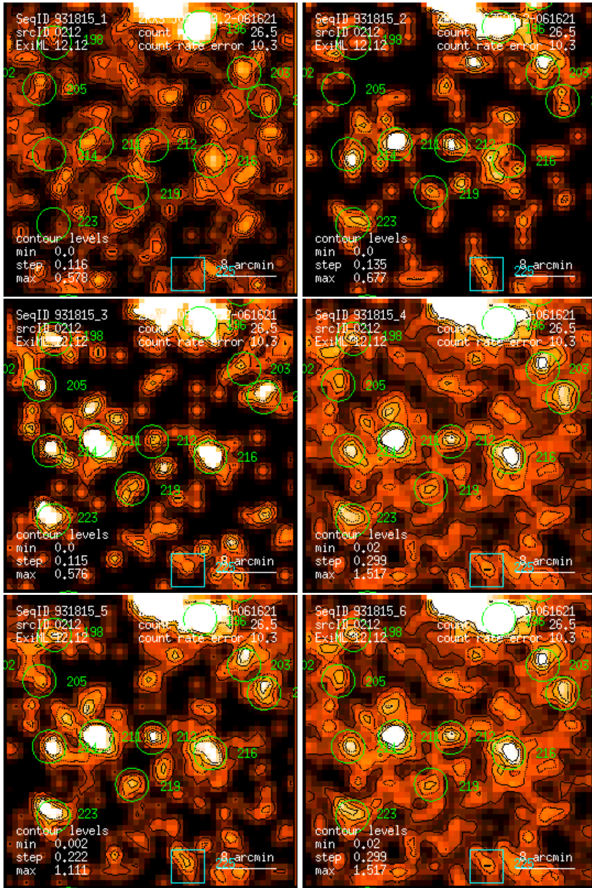
Figure 212: RASS 931815: detection 0212: band rate images, Gaussian filter: (1) PSPC channels 11 – 41, (2) 52 – 90, (3) 91 – 201, (4) 11 – 235, (5) 52 – 201, (6) 11 – 201. Broad band rates in counts/ks. Band rate contour levels in counts/ks/arcmin 2 .
