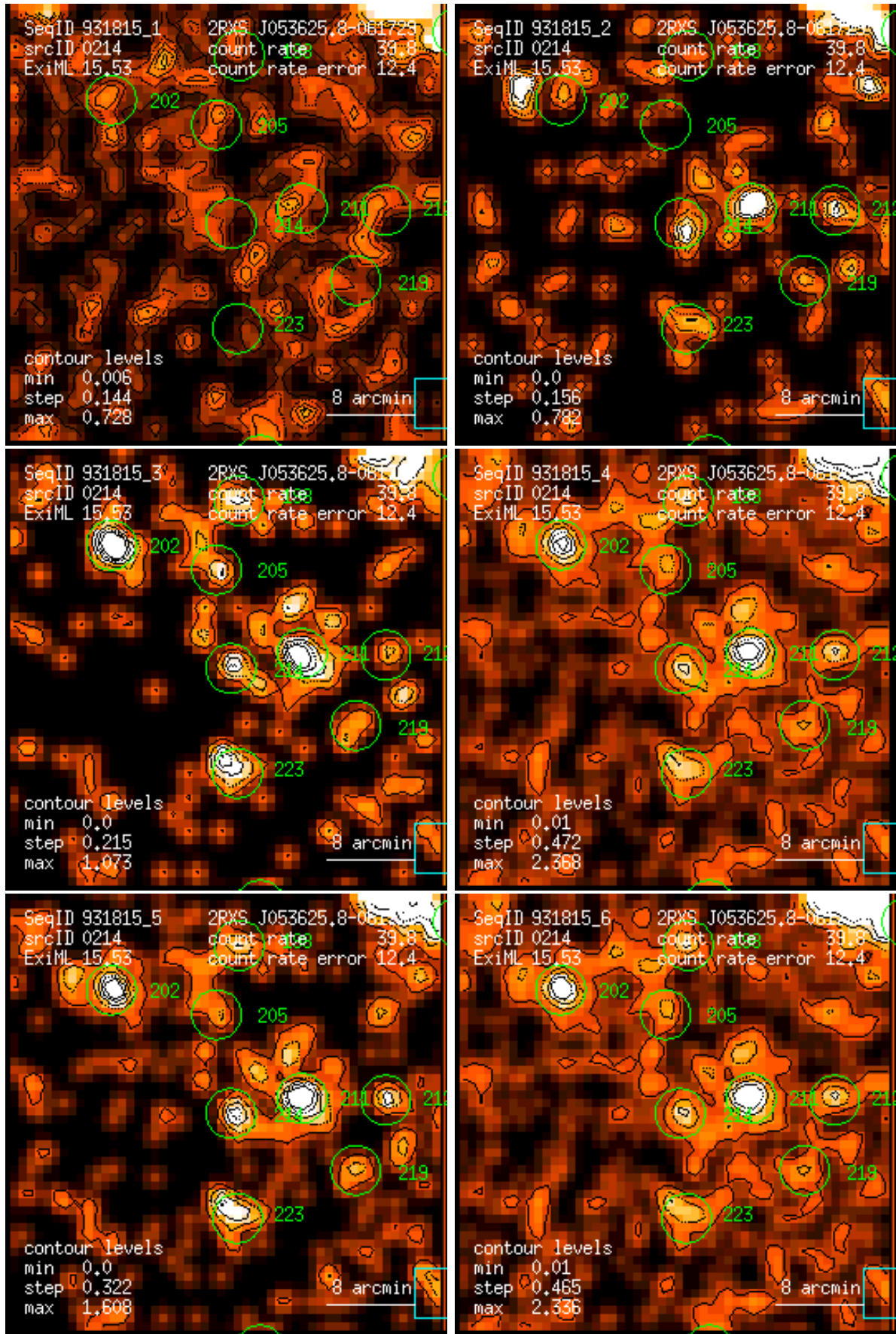
Figure 214: RASS 931815: detection 0214: band rate images, Gaussian filter: (1) PSPC channels 11 – 41, (2) 52 – 90, (3) 91 – 201, (4) 11 – 235, (5) 52 – 201, (6) 11 – 201. Broad band rates in counts/ks. Band rate contour levels in counts/ks/arcmin 2 .
